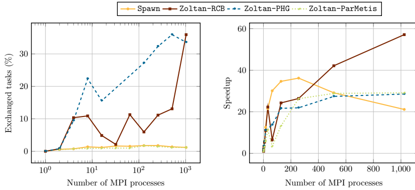
Fig. 11 Resulting data transfer rates (left) and speedups (right) with Zoltan (RCB, PHG), ParMetis (through Zoltan ) and with Spawn . One can notice scalability issues of graph partitioning tools (PHG and ParMETIS ).
