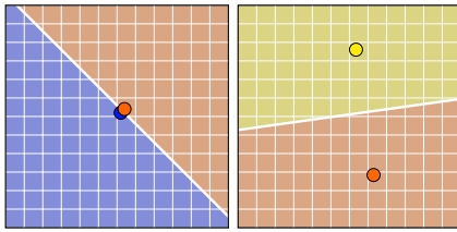
Fig. 6 Left: dipoles formation when using our force equation in its original definition (see equation 6. Right: interactions when using the improved equation version (see equation 7.)
