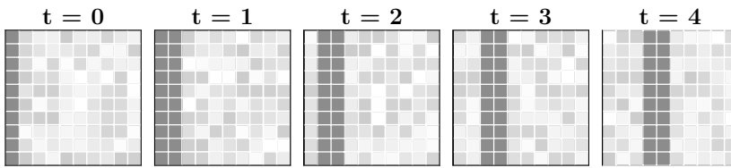
Fig. 8 Generated load evolution: each square represents a task, and the color represents the cost of the task: dark cells are more costly than the white ones, i.e, we do more computations on internal matrices.
