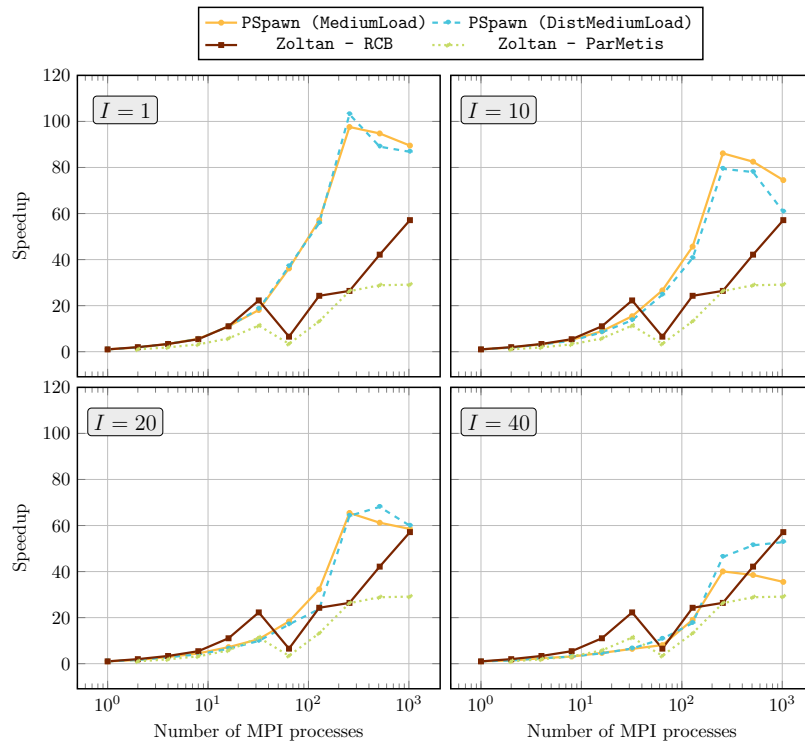
Fig. 12 Cost of the PSpawn iterative model, successively increasing the number of iterations used to compute a partition. Top left: 1 iteration. Top right: 10 iterations. Bottom left: 20 iterations. Bottom right: 40 iterations.
