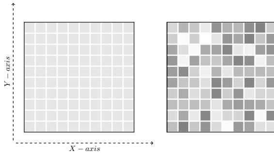
Fig. 4 The task grid model: the grid has a dimension ( x, y, z , with x, y, z \in \mathbb{N} ) and is defined in the Euclidean space. Each cell has a specific coordinate and computing cost (right figure: darker cells have a more important computing cost than white cells).
