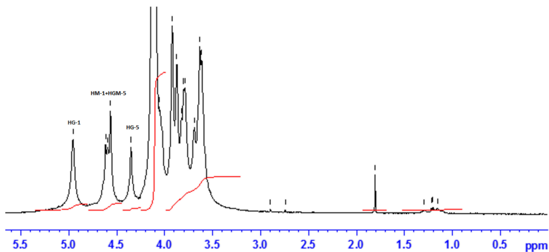
Figure 1. ^1\text{H} NMR spectra of ASBB.
