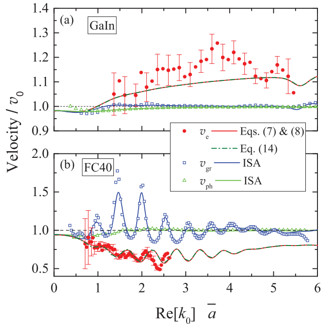
FIG. 11. Frequency dependence of the measured energy velocity in (a) GaIn and (b) FC40 (solid red circles). To highlight the important differences in the energy velocities in these samples, the energy velocities are compared with our data for the phase and group velocities from Figs. 8(b) and 8(c). Theoretical predictions are shown by the solid and dashed lines, as indicated in the legend. Results are normalized by the sound speed in the pure matrix v_0 .
