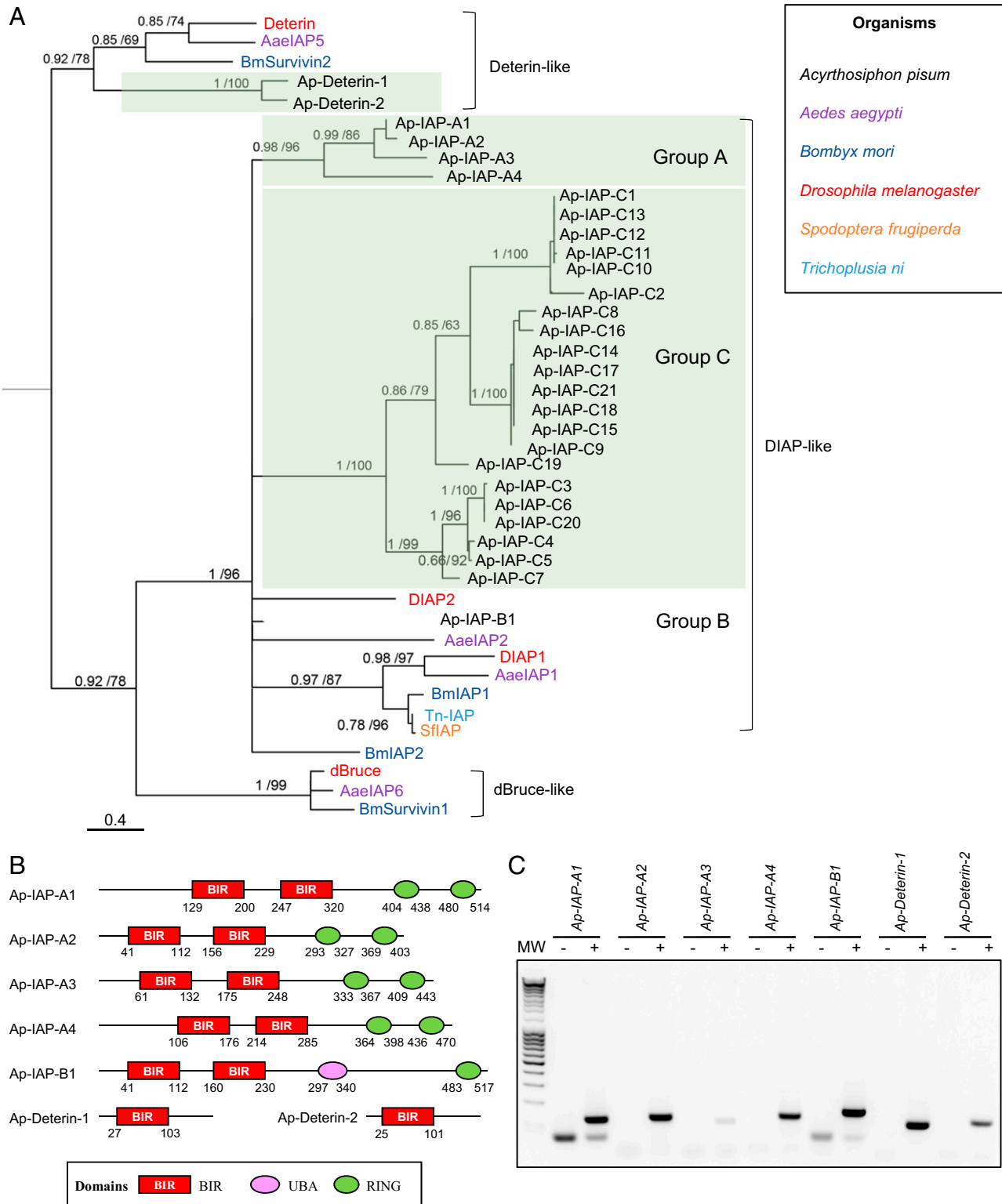
Fig. 2. Identification of IAP-encoding genes in the pea aphid genome. (A) The phylogenetic relationships between IAP protein sequences found in Acyrtosiphon pisum and a selection of insect species based on BIR domain alignment. For each node, Bayesian posterior probability and bootstrap values are indicated. A group of putative A. pisum IAP paralogs are also indicated. This tree was generated using one representative BIR domain from each IAP sequence (full procedure described in the SI Appendix, Supplementary Materials and Methods ). Midpoint rooting was used to present the tree. (B) The domain architecture of selected pea aphid putative IAPs. Each IAP contains at least one BIR domain (Baculoviral IAP Repeat). Additional domains include UBA (ubiquitin-associated domain) and/or RING domains. The positions of amino acids that mark the beginning and the end of the different domains are indicated below each structure. (C) Pea aphid putative IAP genes are expressed. The sequences were successfully amplified from a pool of cDNA obtained from whole aphids at different life stages. For each primer set, a negative control was performed on samples devoid of cDNA. MW, molecular weight marker.
