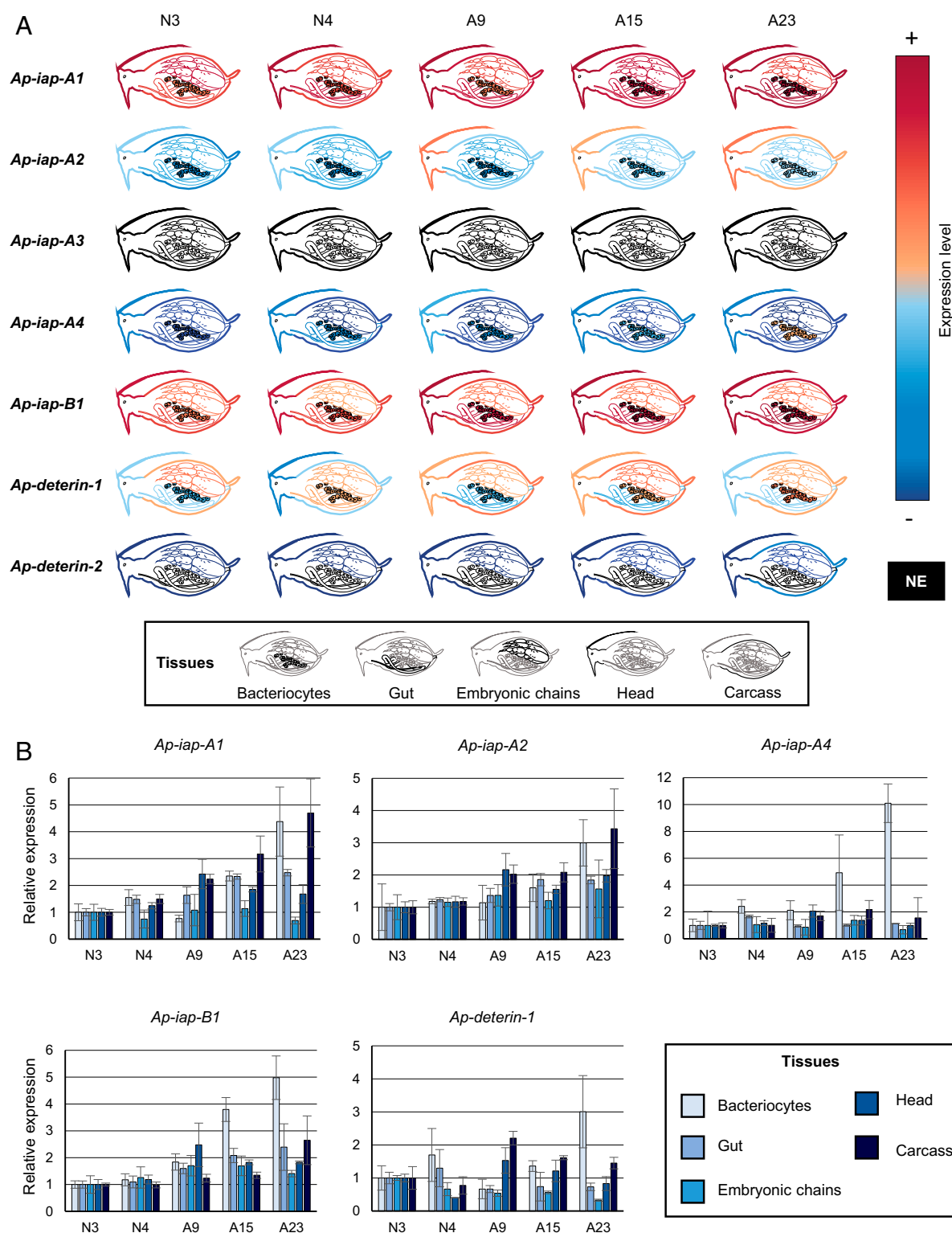
Fig. 3. The expression patterns of pea aphid iap mRNAs across tissues and time. (A) The expression levels of seven selected pea aphid IAPs in different tissues at selected developmental times based on qRT-PCR data analysis. The levels of expression are illustrated by a color scale, going from red (highly expressed) to blue (lowly expressed). Tissues in which the gene is not expressed at a particular time point are represented in black. The expression levels were normalized relatively to the rp17 gene. (B) The expression levels of selected pea aphid IAPs in different tissues throughout aphid development based on qRT-PCR data analysis. iap mRNA gene-expression levels in the different tissues are expressed relative to N3 levels. Data are presented as means \pm SD from three independent biological replicates. mRNA, messenger RNA; NE, not expressed.
