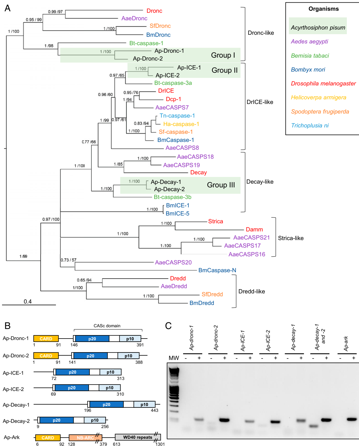
Fig. 1. Identification of caspase- and adaptor protein-encoding genes in the pea aphid genome. (A) The phylogenetic relationships between caspase protein sequences found in Acyrtosiphon pisum and a selection of insect species based on CASc domain alignment. For each node, Bayesian posterior probability and bootstrap values are indicated. A group of putative A. pisum caspase paralogs are also indicated. Midpoint rooting was used to present the tree. (B) The domain architecture of the pea aphid putative caspases and adaptor proteins. Each caspase possesses a CASc domain (CASPase catalytic domain) composed of two distinct subunits (p20 and p10) and preceded by a prodomain of variable size. Ap-Dronc-1 and Ap-Dronc-2 possess an additional CARD domain (Caspase Recruitment Domain) at their N terminus. The putative adaptor protein Ap-Ark contains a CARD domain, a NB-ARC domain, and multiple WD40 repeats. The position of amino acids that mark the beginning and the end of the different domains are indicated below each structure. (C) Pea aphid putative caspases and adaptor proteins genes are expressed. The sequences were successfully amplified from a pool of cDNA obtained from whole aphids at different life stages. For each primer set, a negative control was performed on samples devoid of cDNA. MW, molecular weight marker.
