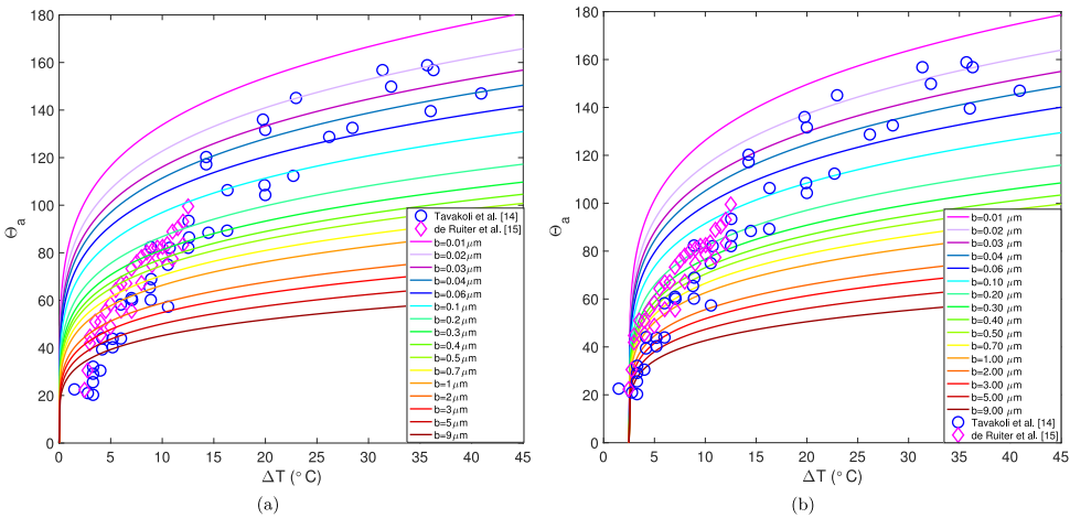
Fig. 5. (a) Apparent angle \theta_a of liquid on substrate, versus undercooling \Delta T , predicted by equation (20). The different curves correspond to different values of the mesoscopic cut-off length b , ( a is set to 0.845 nm). Data points are experiments from de Ruiter et al. [15] and from Tavakoli et al. [14]. (b) Same as (a) with an offset in temperature added in equation (20), \Delta T_c = 2.46^\circ .
