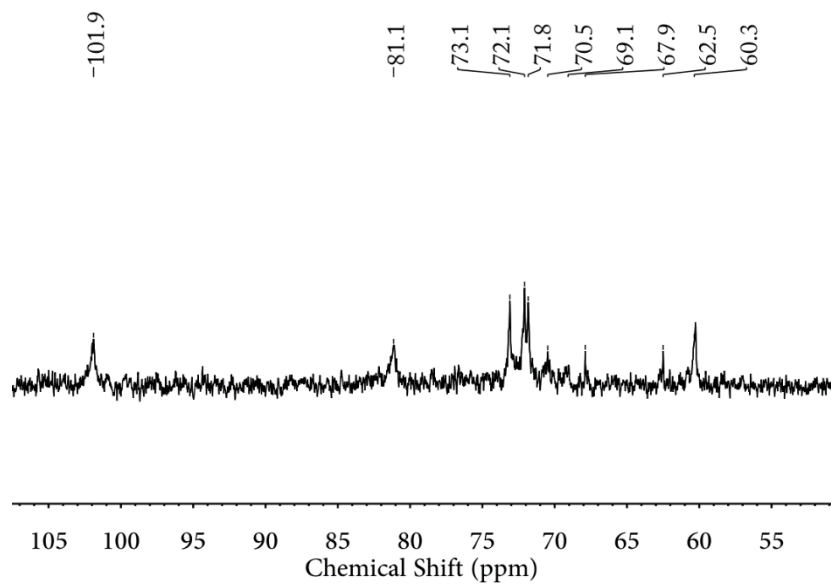
Figure S1. ^{13}\text{C} NMR spectrum of PCD (100 MHz, \text{D}_2\text{O} ).
