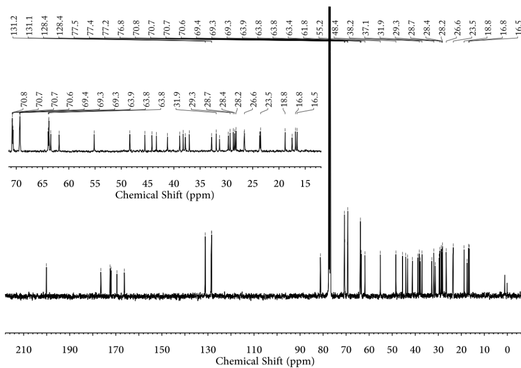
Figure S10. ^{13}\text{C} NMR spectrum of GADA (100 MHz, \text{CDCl}_3 )
