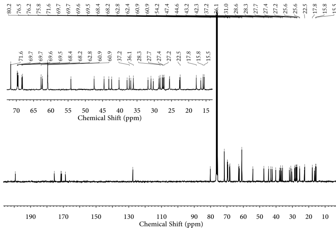
Figure S7. ^{13}\text{C} NMR spectrum of GA-OEG (100 MHz, \text{CDCl}_3 )
