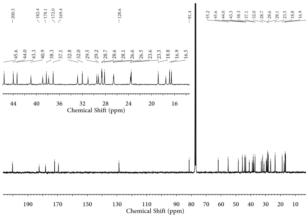
Figure S4. ^{13}\text{C} NMR spectrum of GAA (100 MHz, \text{CDCl}_3 )
