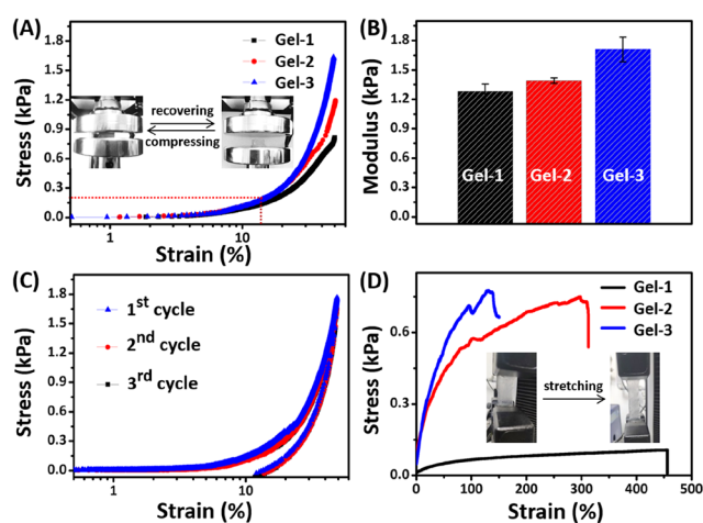
Figure 5. (A) Mechanical compression curves of Gel-1, Gel-2 and Gel-3, and (B) their responding compression modulus. (C) Cyclic compression curves of Gel-3. (D) Mechanical tensile curves of Gel-1, Gel-2 and Gel-3.
