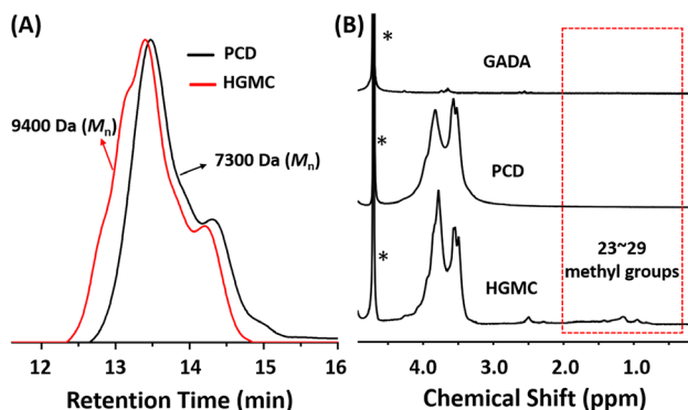
Figure 2. (A) SEC spectra of PCD and HGMC with refractometer as detector (DMF as eluent, polystyrene standards for molecular weights calibration). (B) 1 H NMR spectra of GADA (up), PCD (middle) and HGMC (bottom) in D 2 O (400 MHz). *represents the solvent peak.
