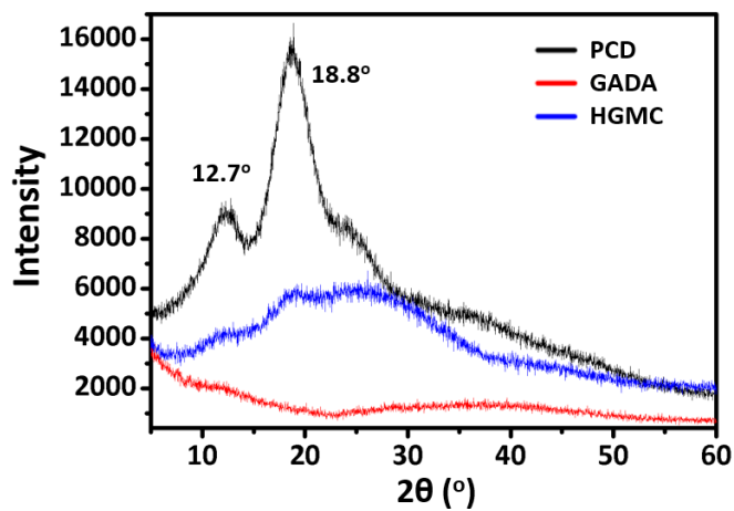
Figure S2. X-ray diffraction patterns of PCD, GADA and HGMC.
