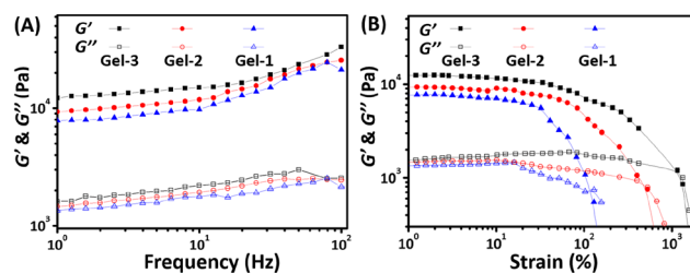
Figure 4. (A) Oscillatory frequency sweep of Gel-1, Gel-2 and Gel-3 at a strain 1%; (B) G' and G'' of Gel-1, Gel-2 and Gel-3 as a function of strain at a frequency of 1 Hz.
