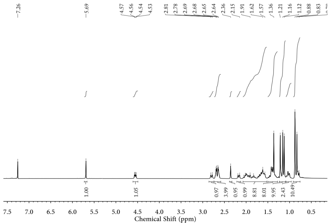
Figure S3. ^1\text{H} NMR spectrum of GAA (400 MHz, \text{CDCl}_3 )
