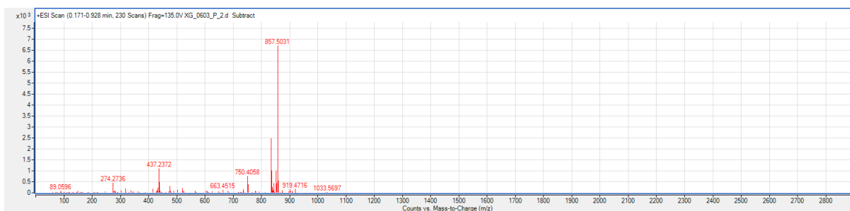
Figure S8. HRMS-ESI (+) spectrum of GA-OEG
