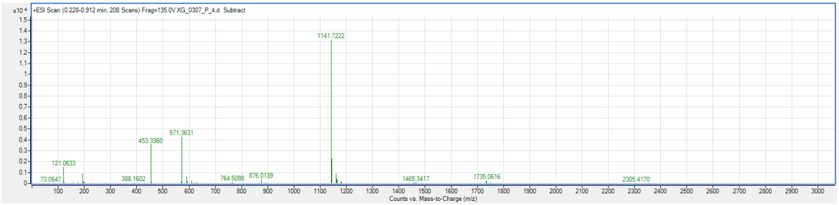
Figure S5. HRMS-ESI (+) spectrum of GAA
