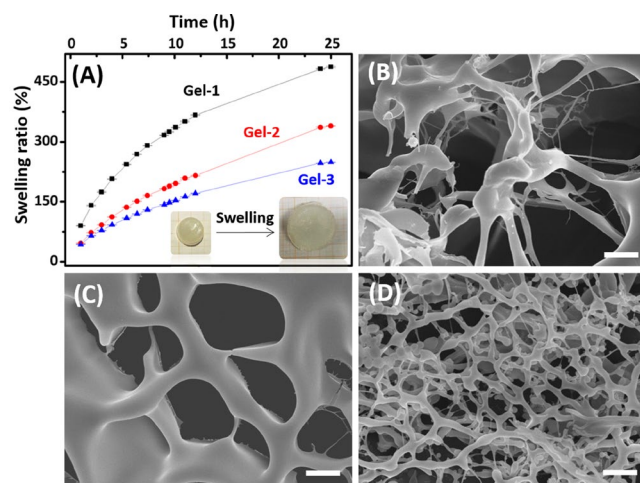
Figure 3. (A) Swelling behaviors and (B, C, D) SEM images of Gel-1, Gel-2 and Gel-3. Scale bar is 2 μm for (B), (C) and (D).
