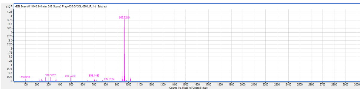
Figure S11. HRMS-ESI (+) spectrum of GADA
