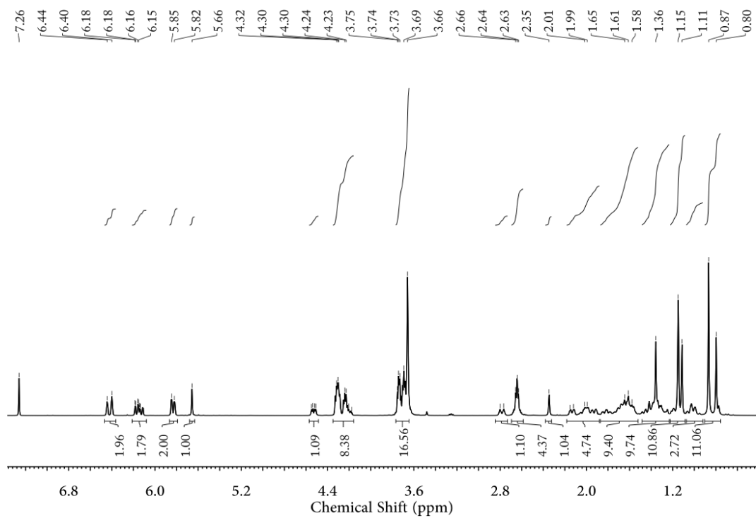
Figure S9. ^1\text{H} NMR spectrum of GADA (400 MHz, \text{CDCl}_3 )
