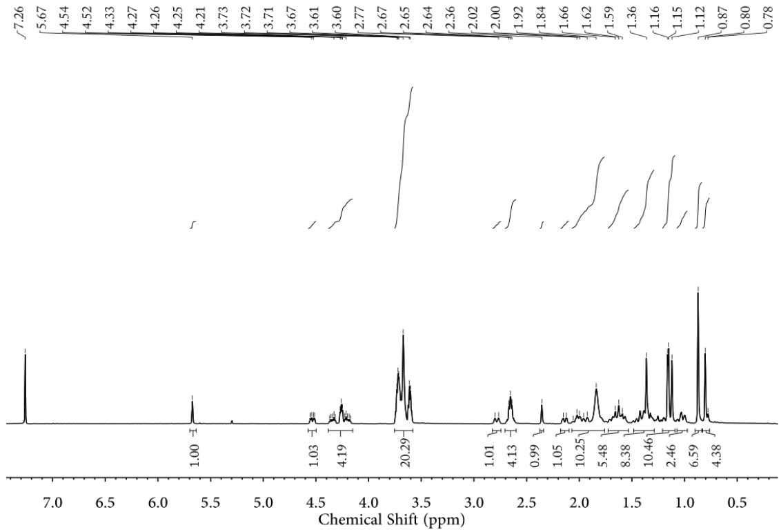
Figure S6. ^1\text{H} NMR spectrum of GA-OEG (400 MHz, \text{CDCl}_3 )
