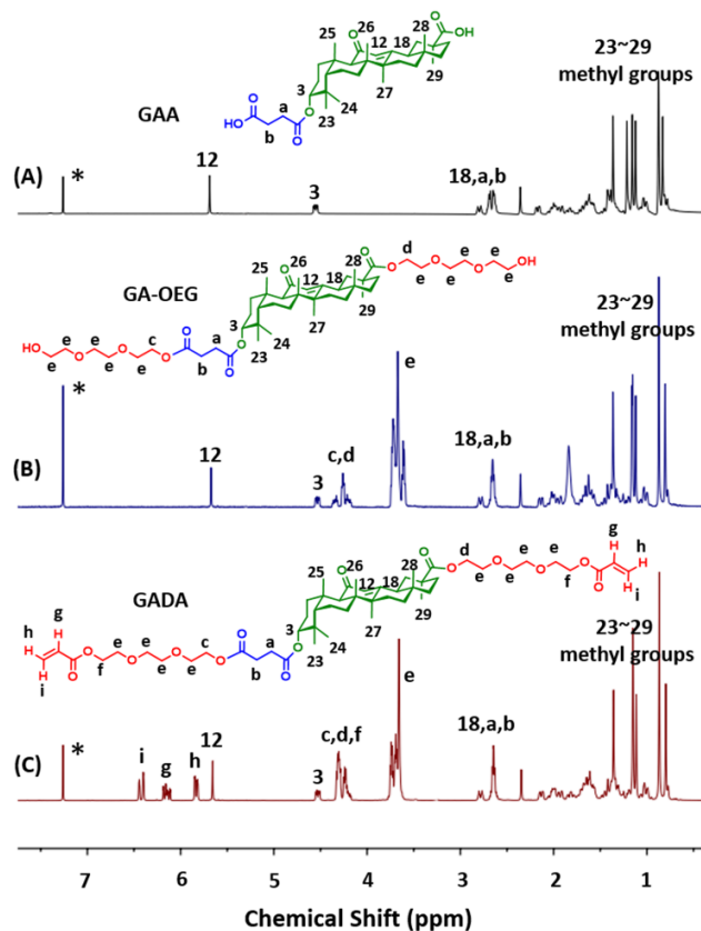
Figure 1. ^1\text{H} NMR spectra of (A) GAA, (B) GA-OEG and (C) GADA (400 MHz, \text{CDCl}_3 ). *represents the solvent peak.
