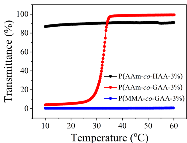
Fig. S3. Transmittance of the aqueous solutions of P(AAm-co-GAA-3%), P(AAm-co-HAA-3%), and P(MMA-co-GAA-3%) as a function of temperature at a wavelength of 450 nm and a cooling rate of 1.0 °C/min at the concentration of 15 mg/mL.
