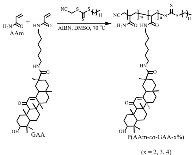
Scheme 1. Illustration of copolymerization of natural glycyrrhetic acid-derived acrylamide (GAA) with acrylamide (AAm).
