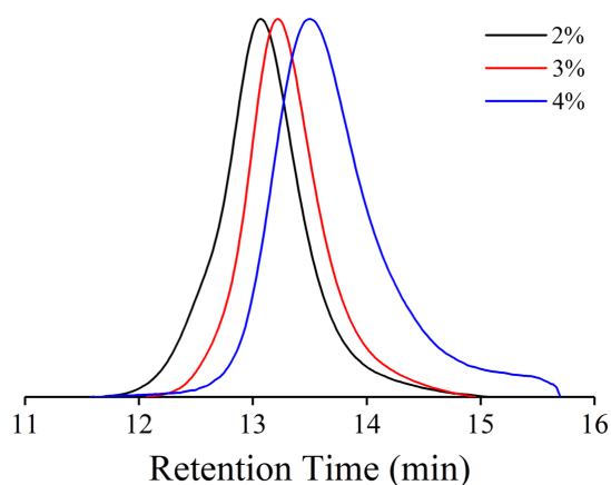
Fig. S1. SEC spectra of P(AAm- co -GAA- x %) ( x = 2, 3, 4) with refractometer as detector (DMSO as eluent, dextran standards for molecular weight calibration). The right shoulder peak of P(AAm- co -GAA-4%) was mainly due to the formation of trace oligomers.
