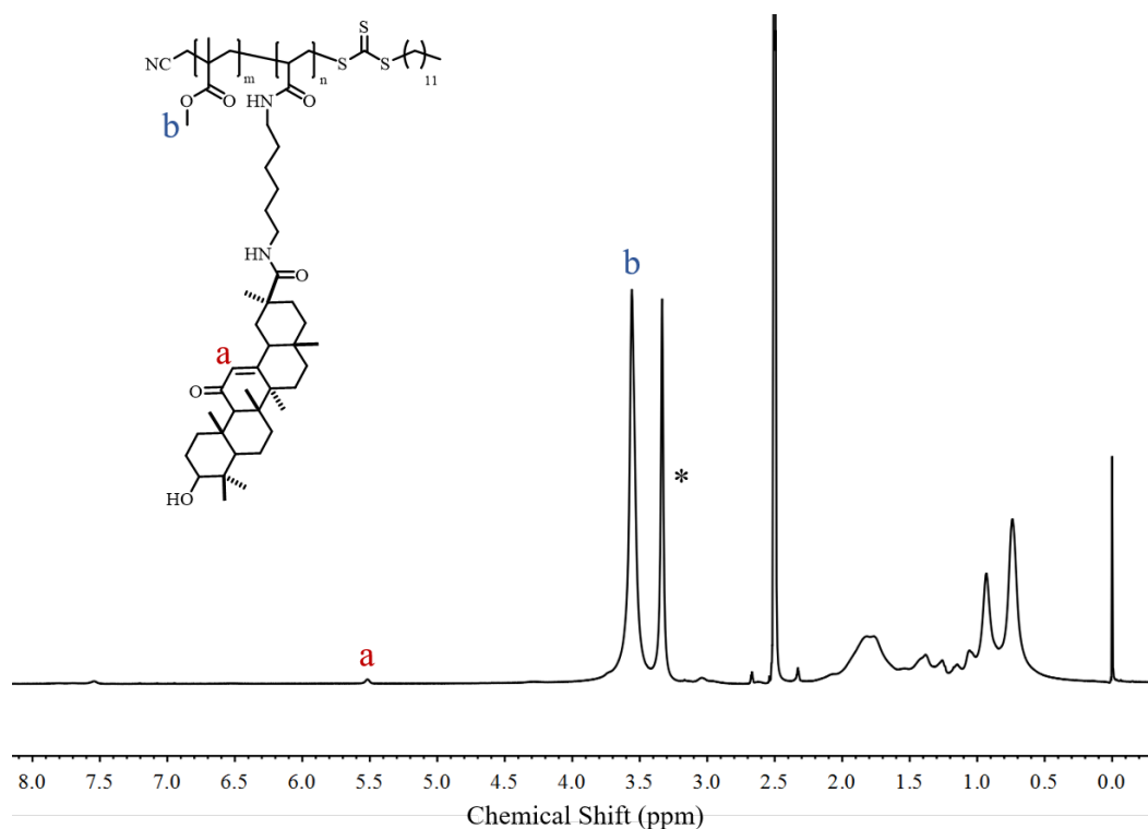
Fig. S23. ^1\text{H} NMR spectrum of copolymer P(MMA- co -GAA-3%) (400 MHz, d_6 -DMSO). “*” means water.
