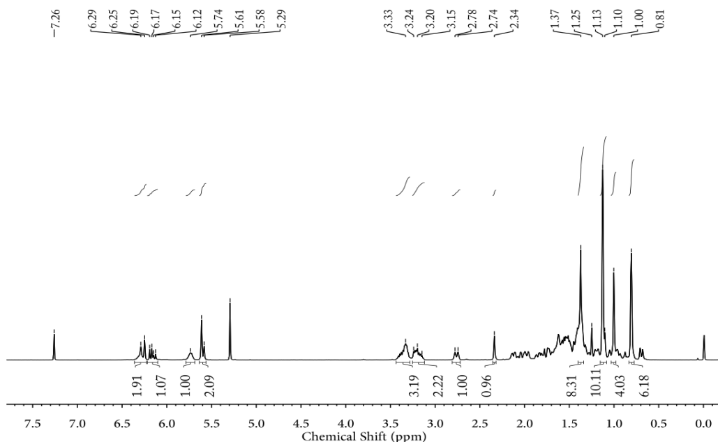
Fig. S13. ^1\text{H} NMR spectrum of GAA (400 MHz, \text{CDCl}_3 )
