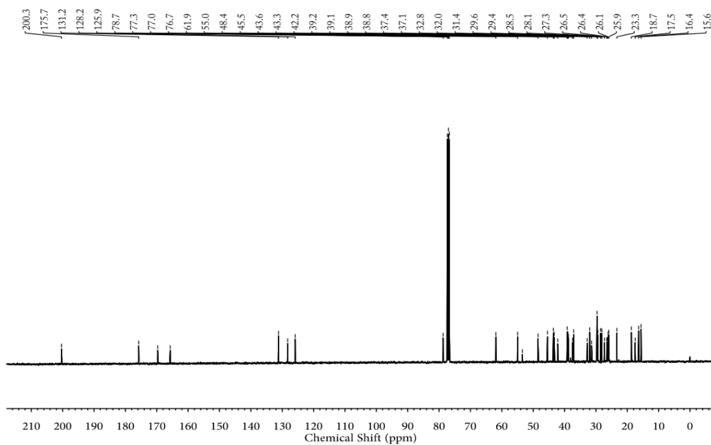
Fig. S14. ^{13}\text{C} NMR spectrum of GAA (100 MHz, \text{CDCl}_3 )
