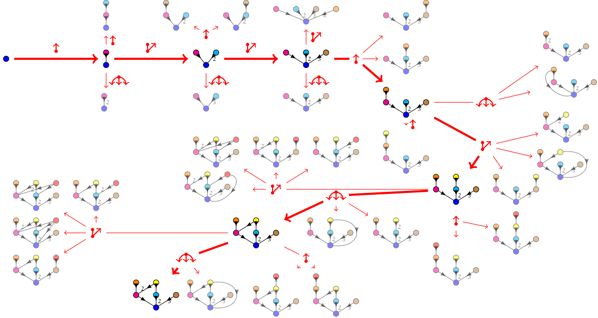
Figure 2: The path (in bold) in the FDAG enumeration tree that leads to the construction of the FDAG presented in Figure 1. The expansions rules are denoted with symbols (\uparrow) , (\nearrow) and (\curvearrowright) .
