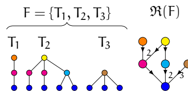
Figure 1: A forest F (left) and its DAG reduction (right).
