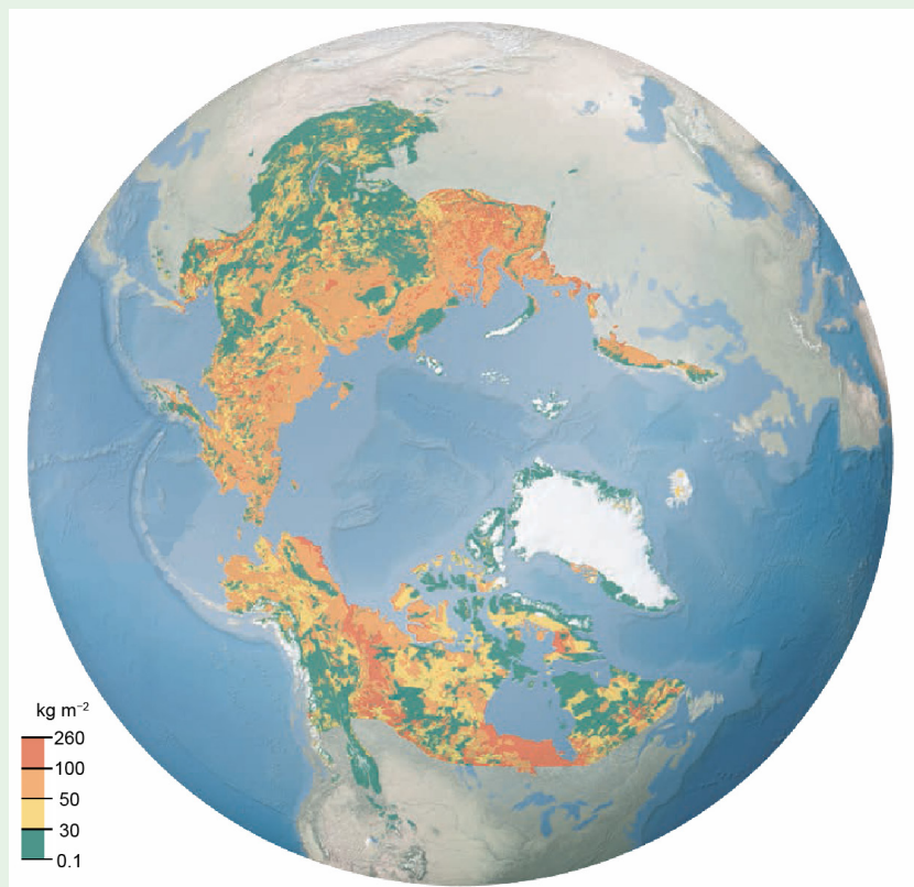
Fig. SB5.3. Soil organic carbon pools ( \text{kg m}^{-2} ; 0–3 m depth) for the northern circumpolar permafrost region. (Modified from Scientific American , Nov 2016.)
