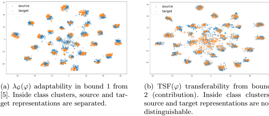
Fig. 1: TSNE [32] visualisation of representations when trained to minimize (a) adaptability error \lambda_G(\varphi) from [5], (b) transferability error \text{TSF}(\varphi) introduced in the present work. The task used is A \rightarrow W of the Office31 dataset. Labels in the target domain are used during learning in this specific experiment. For both visualisations of representations, we observe well-separated clusters associated to the label classification task. Inside those clusters, we observe a separation between source and target representations for \lambda_G(\varphi) . That means that representations embed domain information and thus are not invariant. On the contrary, source and target representations are much more overlapping inside of each cluster with \text{TSF}(\varphi) , illustrating that this new term is not conflictual with invariance.
