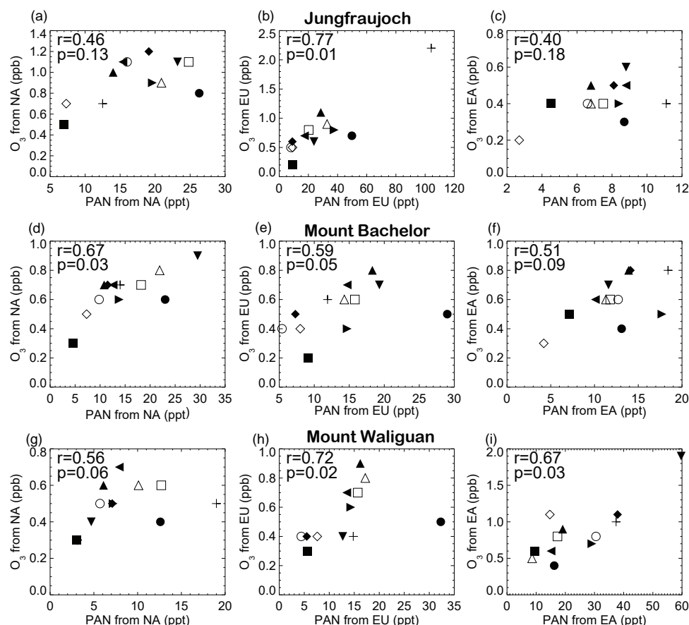
Figure 7. SRRs for O 3 versus PAN at Jungfraujoch (a, b, c), Mount Bachelor (d, e, f), and Mount Waliguan (g, h, i), obtained by subtracting the SR6XX from the SR1 simulations (Table 2) available from 12 models, for which XX denotes the NA (a, d, g), EU (b, e, h), or EA (c, f, i) source region. Each model thus contributes one point (symbols defined in Table 1) in each panel. Spearman's (rank) correlation coefficient and p values are also shown.
