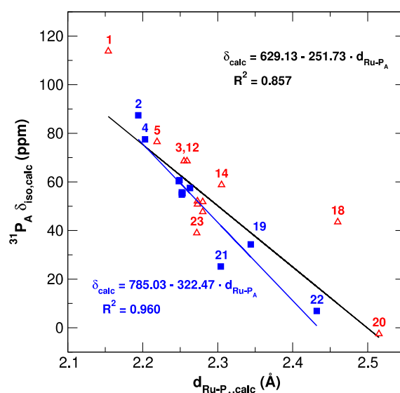
Figure 3. Calculated chemical shifts \delta^{\text{P}_A} (ppm) vs. calculated Ru- \text{P}_A distances (Å). The blue full squares and red empty triangles correspond to observed and non-observed isomers, respectively. For labelling of complexes, see Table 1.
