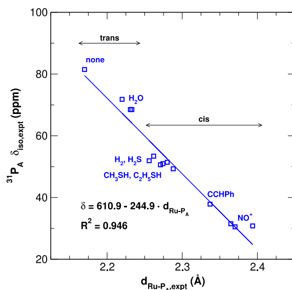
Figure 1. Plot of ^{31}\text{P}_A\{\text{H}\} experimental data vs. experimental \text{Ru-P}_A bond length ( \text{\AA} ) for \text{RuCl}_2(\text{P}_A\text{-N})[\text{P}(p\text{-tolyl})_3] and the \text{RuX}_2(\text{P}_A\text{-N})(\text{PR}_3)\text{L} complexes, where \text{X} = \text{Cl} or \text{Br} , and \text{R} = \text{Ph} , p\text{-tolyl} or p\text{-FC}_6\text{H}_4 ; \text{L} is shown in Scheme 1; various crystalline forms are included when occurring; none is \text{RuCl}_2(\text{P}_A\text{-N})[\text{P}(p\text{-tolyl})_3] .
