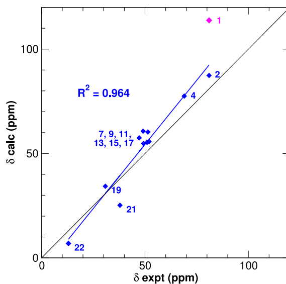
Figure 2. Calculated vs. experimental ^{31}P_A chemical shifts for RuCl_2(P_A-N)(PR_3)L . See Table 1 for labelling of the complexes. The reference value for calculating ^{31}P chemical shifts is 351.6 ppm. 32
