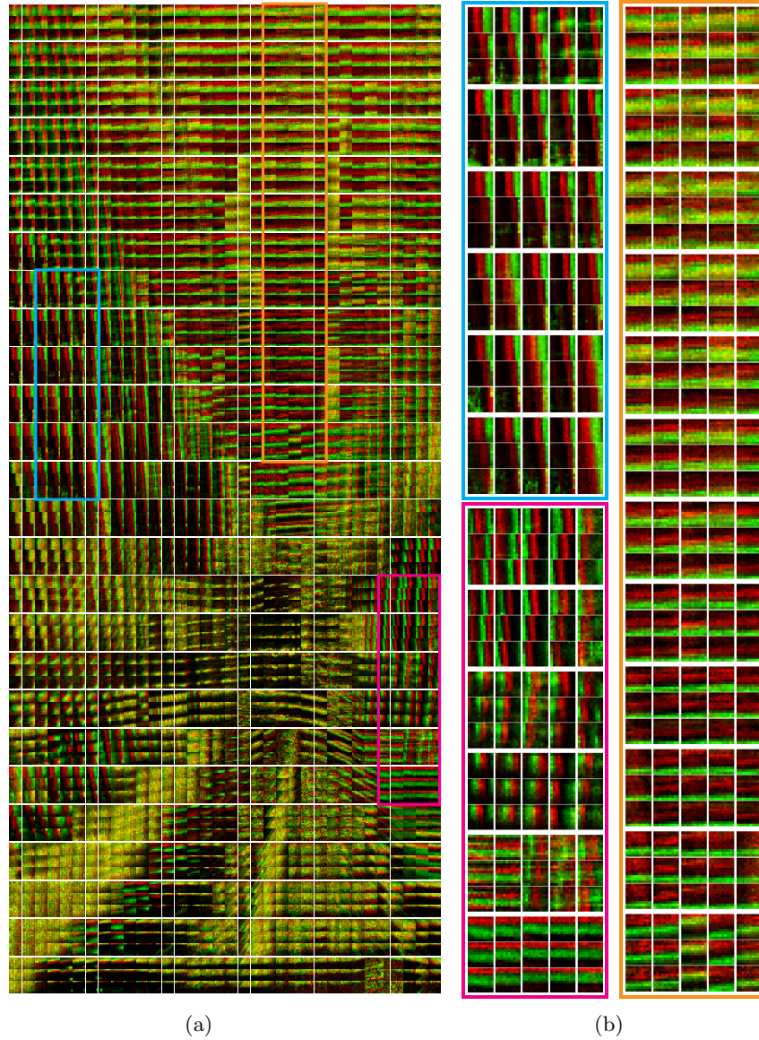
Fig. 5: Motion tuned receptive fields learned at different image locations. (a) Receptive fields learned across the entire field of view. Each receptive field has three sub-fields (arranged vertically) corresponding to different synaptic delays. (b) Enlarged view of marked groups of receptive fields in (a). See text for details.
