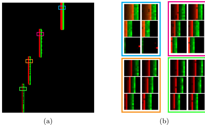
Fig. 4: Motion sensitive receptive fields develop from STDP with multiple synaptic delays. (a) On and off events recorded by the DV-software visualisation GUI for 4 vertical bars moving at speeds of 420, 210, 140 and 105 px/s (top to bottom). (b) Receptive fields of pairs of neighboring neurons receiving the 4 vertical bars as input (arranged by decreasing speed from top left to bottom right). Each neuron has 3 groups of input synapses with delays of 0, 10, and 20 ms (top to bottom). The expected displacements of the 4 bars during 10 ms are 4.2, 2.1, 1.4 and 1.05 pixels, which matches the horizontal shifts of receptive field structures for different synaptic delays.
