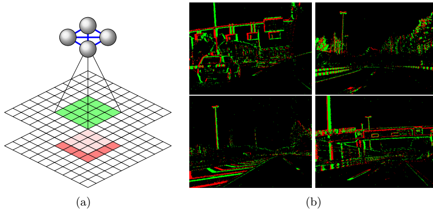
Fig. 1: (a) Groups of N = 4 neurons are connected to the same patch of input pixels providing On (green) and Off (red) events. The neurons are linked by inhibitory connections (blue). A neuron can be connected to pixels of its receptive field by D synapses with different delays to gain localised motion sensing properties (not shown). (b) Examples of input events from the driving sequence.
