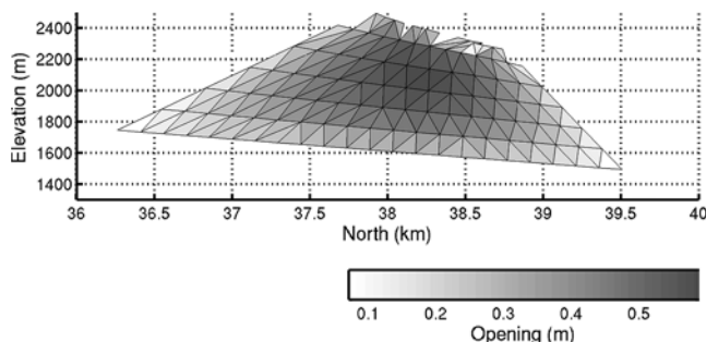
Figure 15. Opening of the dike in response to the constant overpressure for the maximum PPD model. The maximum opening is 59 cm, the average on the whole area and that on the ground surface are 35 and 25 cm, respectively.
