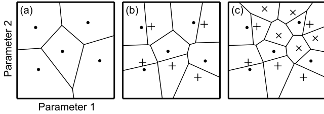
Figure 5. Example showing the search process, in the case n = 5 in two model dimensions. (a) Initial. Five initial models (dots) are randomly generated, and Voronoi cells are defined. (b) First iteration. Five new models (pluses) are generated in the Voronoi cells around the five best models (in this case, in every initial cell), and new Voronoi cells are defined. (c) Second iteration. Five new models (crosses) are generated around the five best models, and new Voronoi cells are defined. Note that the newly generated points modify the shapes of the surrounding cells.
