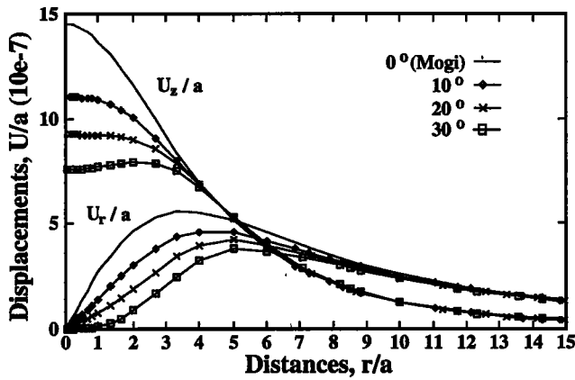
Figure 2. Surface displacements created by a spherical pressure source beneath volcanoes with average slopes of 0°, 10°, 20° and 30°. Poisson's ration is 0.21, and Young's modulus is 50 GPa. Displacements and distances are normalized by source radius.
