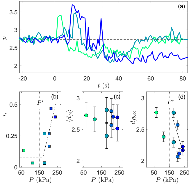
FIG. 11. Influence of the acoustic pressure P on TRUSAXS spectra. (a) Exponent p of the best power-law fit I(q) \sim q^{-p} at low q as a function of time. Ultrasound with frequency 20 kHz is turned on at time t = 0 and switched off at t = 30 s. Each curve corresponds to a given acoustic pressure P = 64 (green), 160 (blue-green) and 240 kPa (blue). (b) Intermittency index i_i as a function of P . (c) Micro-cracks average interfacial fractal dimension \langle d_{fi} \rangle as a function of P . (d) Bulk fractal dimension of the gel d_{fb,\infty} measured 40 s after ultrasound are turned off as a function of P .
