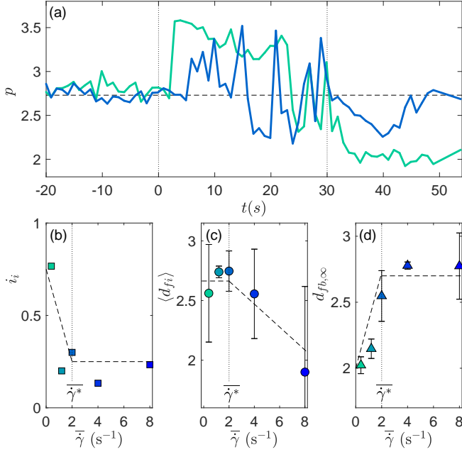
FIG. 14. Influence of the shear rate on the TRUSAXS spectra of gels exposed to high-power ultrasound. (a) Exponent p of the best power-law fit I(q) \sim q^{-p} at low q as a function of time. Ultrasound with frequency 20 kHz and pressure P = 240 kPa is turned on at time t = 0 and switched off at t = 30 s. A mean shear rate \bar{\gamma} across the flow cell is applied during the whole experiment. The green and blue curves correspond to \bar{\gamma} = 0.4 and 2 s ^{-1} respectively. (b) Intermittency index i_i as a function of \bar{\gamma} . (c) Micro-cracks average interfacial fractal dimension \langle d_{fi} \rangle as a function of \bar{\gamma} . (d) Bulk fractal dimension of the gel d_{fb,\infty} measured 20 s after ultrasound are turned off as a function of \bar{\gamma} . For \bar{\gamma} = 4 and 8 s ^{-1} , due to the large flow rate imposed by the syringe pump, the gel that passes across the X-ray beam has no longer received any ultrasound at t \simeq 50 s, i.e., 20 s after ultrasound are turned off. We therefore measure d_{fb,\infty} on the longest possible time after ultrasound is turned off while the gel has received ultrasound, respectively 4.5 s and 1.5 s for \bar{\gamma} = 4 and 8 s ^{-1} .
