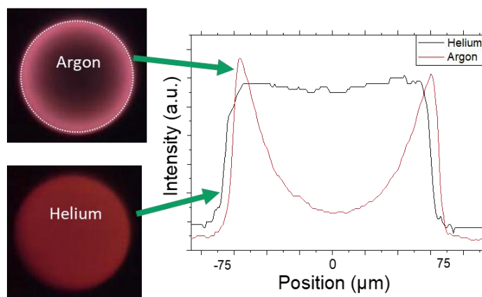
Fig. 1: Images of a micro discharge in single hole configuration operated in argon and helium at atmospheric pressure with a maximum current of 0,8mA. (Micro reactor configuration : single hole, diameter 150 μm, depth 55 μm)
