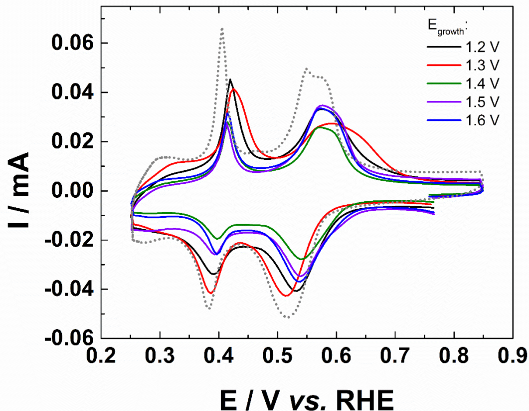
Figure 8: Voltammetric upd profiles of AuNPs in 0.1 mol L -1 NaOH + 1 mmol L -1 Pb(NO 3 ) 2 recorded at 20 mV s -1 and at a temperature of 20 °C after polarization at E growth . Dashed line represents upd profile without the oxide growth step.
