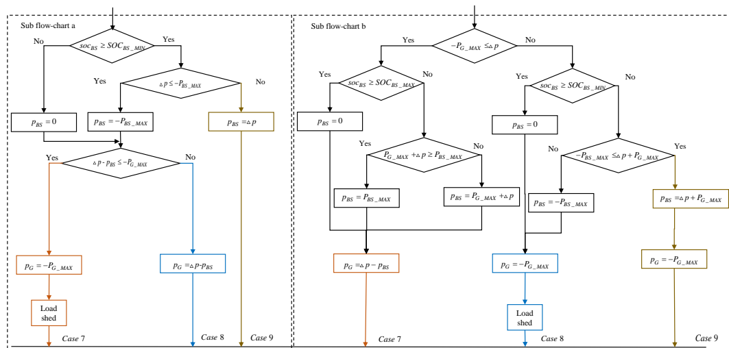
Figure 5. Sub-flowchart a and sub-flowchart b.
