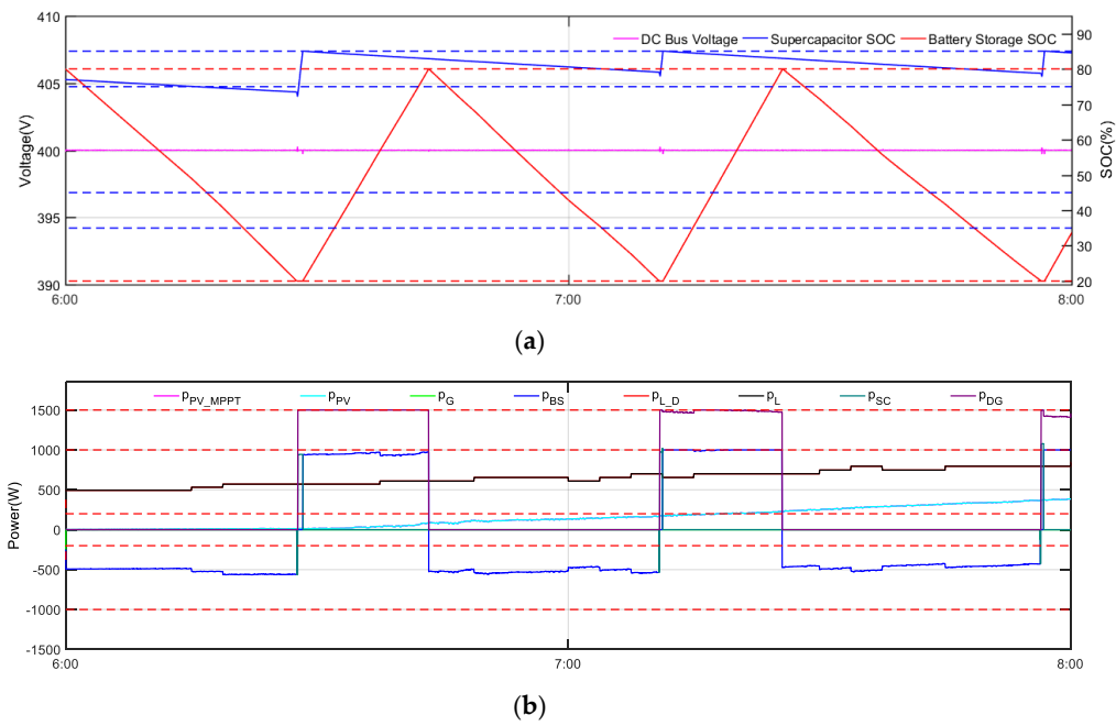
Figure 10. Curves of common DC Bus voltage and SOC of storage (a) and curves of power (b) during the period 6:00–8:00.
