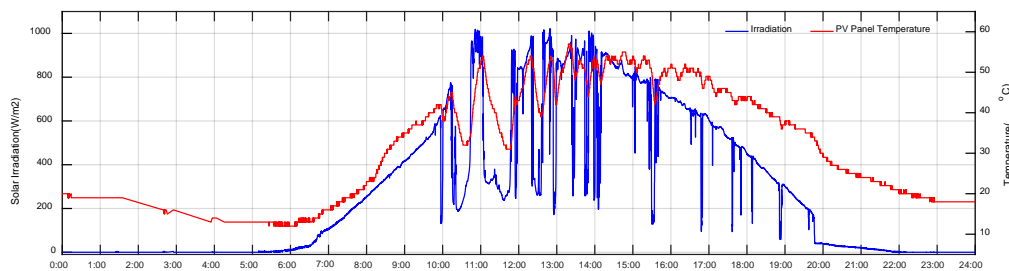
Figure 6. Weather data on the 20th June 2018 in Compiègne, France.
