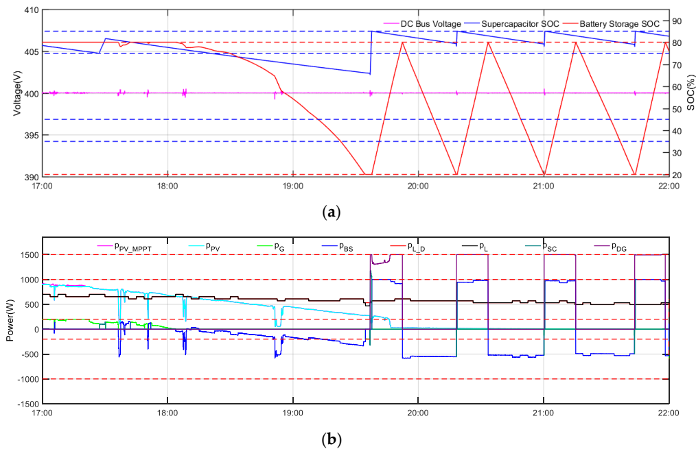
Figure 16. Curves of common DC bus voltage and SOC of storage (a) and curves of power (b) during the period 17:00–22:00.
