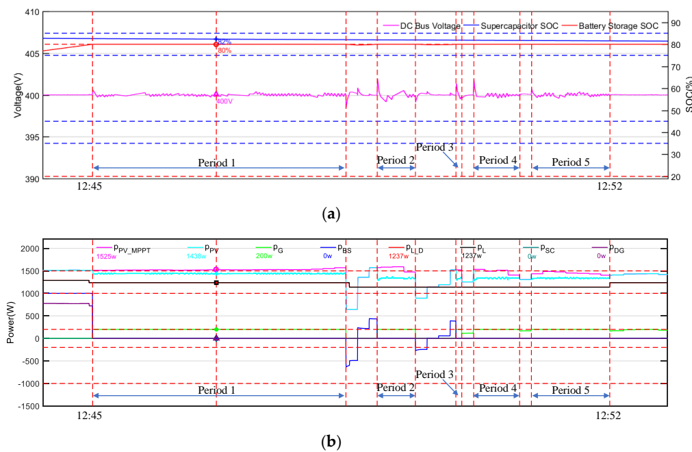
Figure 14. Curves of common DC Bus voltage and SOC of storage (a) and curves of power (b) during PV shedding.
