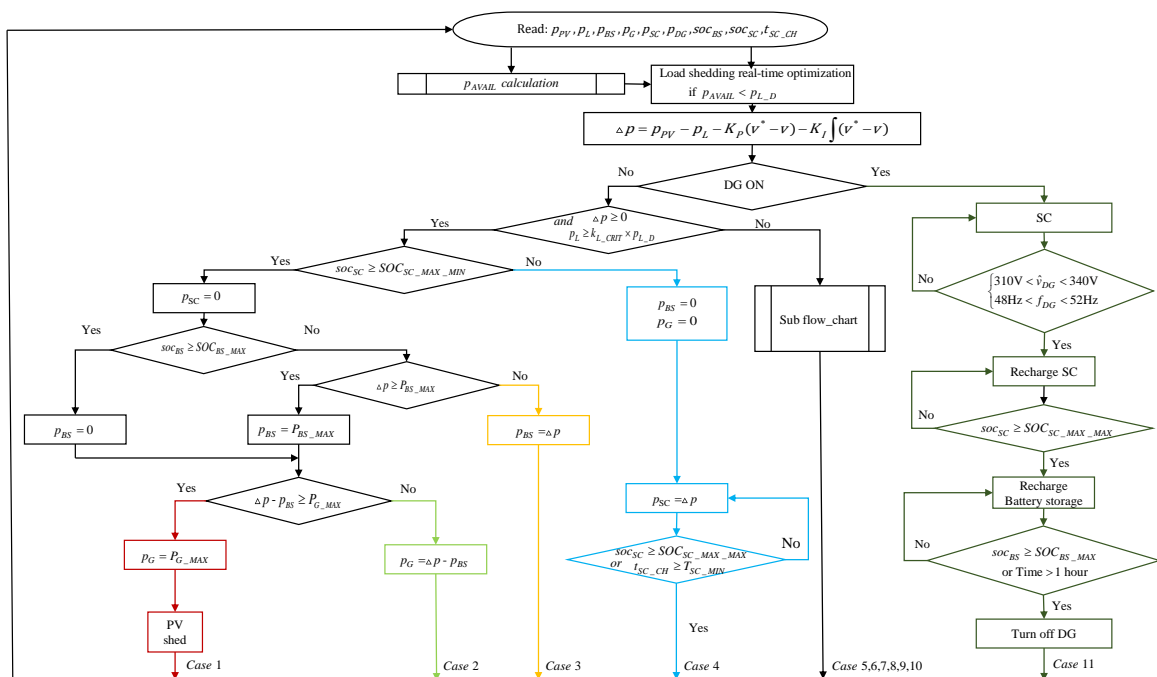
Figure 2. Flowchart of operational power control and management algorithm.
