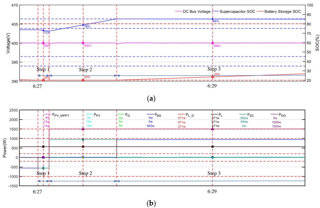
Figure 11. Curves of common DC Bus voltage and SOC of storage (a) and curves of power (b) when the diesel generator (DG) is turned on.
