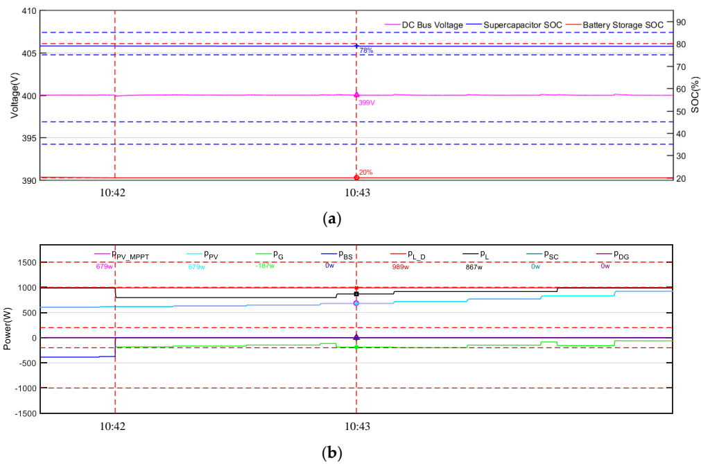
Figure 13. Curves of common DC bus voltage and SOC of storage (a) and curves of power (b) during load shedding.
