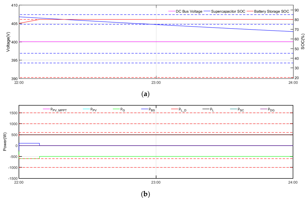
Figure 17. Curves of common DC bus voltage and SOC of storage (a) and curves of power (b) during the period 22:00–24:00.
