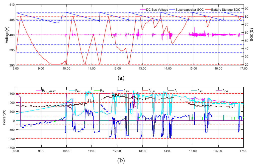
Figure 12. Curves of common DC bus voltage and SOC of storage (a) and curves of power (b) during the period 8:00–17:00.
