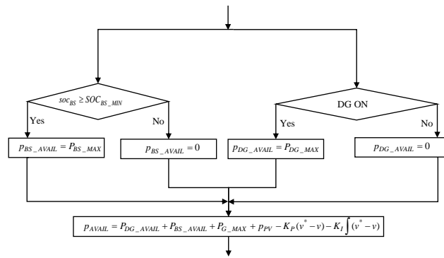
Figure 3. Flowchart of available power calculation.
