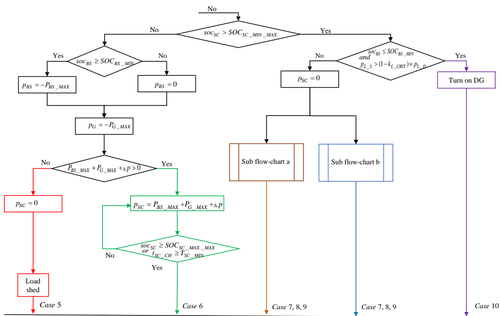
Figure 4. Sub-flowchart of operational power control and management algorithm.
