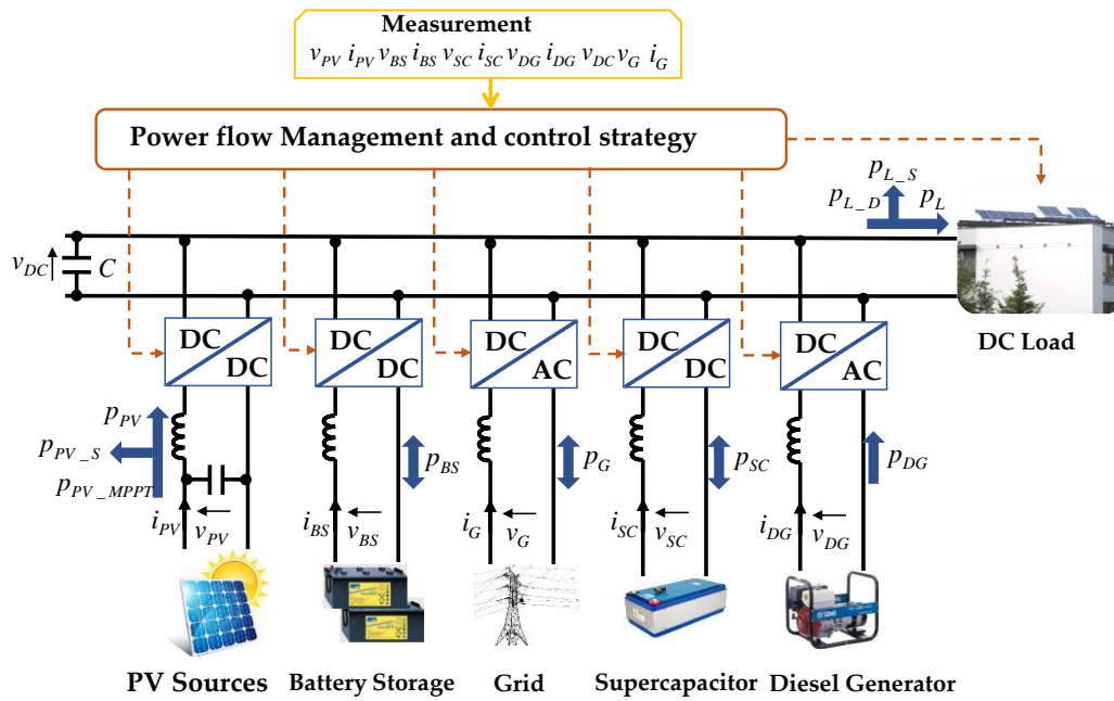
Figure 1. Overview of full direct current (DC) microgrid.
