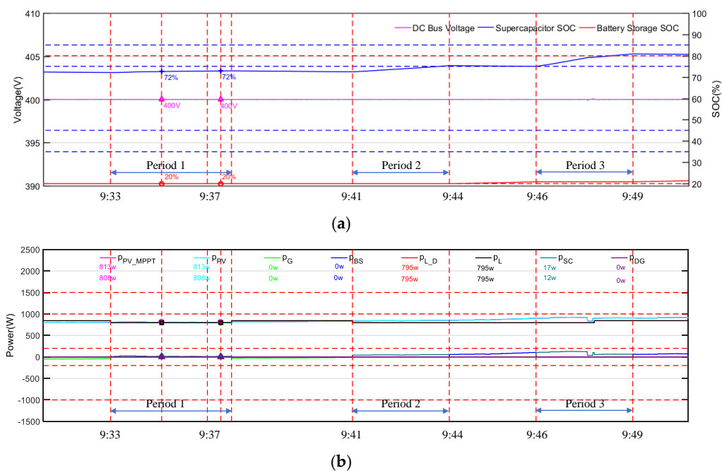
Figure 15. Curves of common DC bus voltage and SOC of storage (a) and curves of power (b) during SC recharging.
