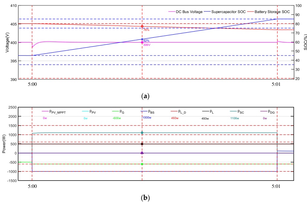
Figure 9. Curves of common DC bus voltage and SOC of storage (a) and curves of power (b) while the supercapacitor (SC) is recharging.
