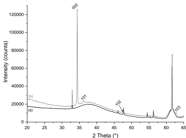
Figure 1 : XRD patterns of (a) silicon wafer and (b) ZnO NWs grown on Si wafer.
