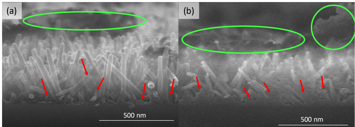
Figure 7 : Cross-sectional SEM images of ZnO/YAG:Ce composite coatings made with (a)5 and (b) 20 impregnations of YAG:Ce NPs suspension. Red arrows indicate YAG:Ce NPs lying between ZnO NWs whereas green circles highlight the surface crust.
