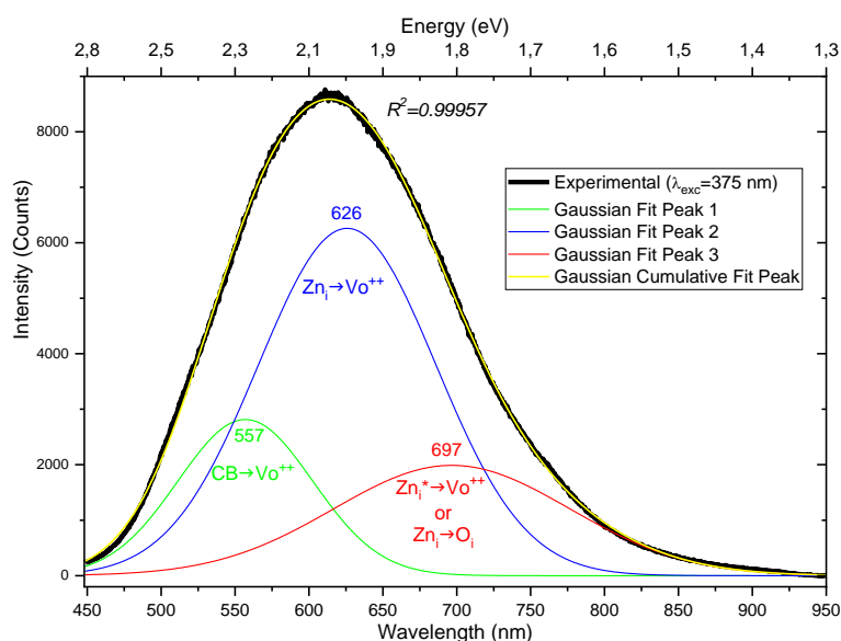
Figure 10: Room temperature emission spectrum of ZnO NWs alone associated with its decomposition into three Gaussian components and their cumulative signal.
