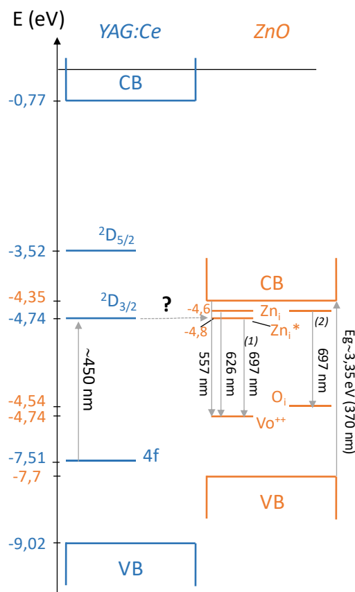
Figure 11 : Schematic energy levels diagram based on one hand on the work of Merenga et al. [60] for YAG:Ce, and on the other hand both on the work of Tzeng et al. [59] and on the deconvoluted emission spectrum recorded in this work under 375 nm (Figure 10) for ZnO NWs.
