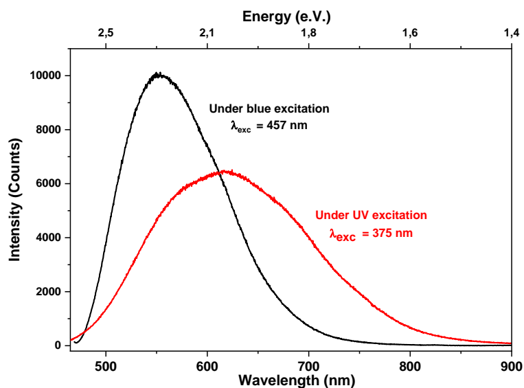
Figure 13 : Room temperature emission spectra of a YAG :Ce/ZnO NWs composite coating prepared with 15 impregnations of ground YAG:Ce suspension.
