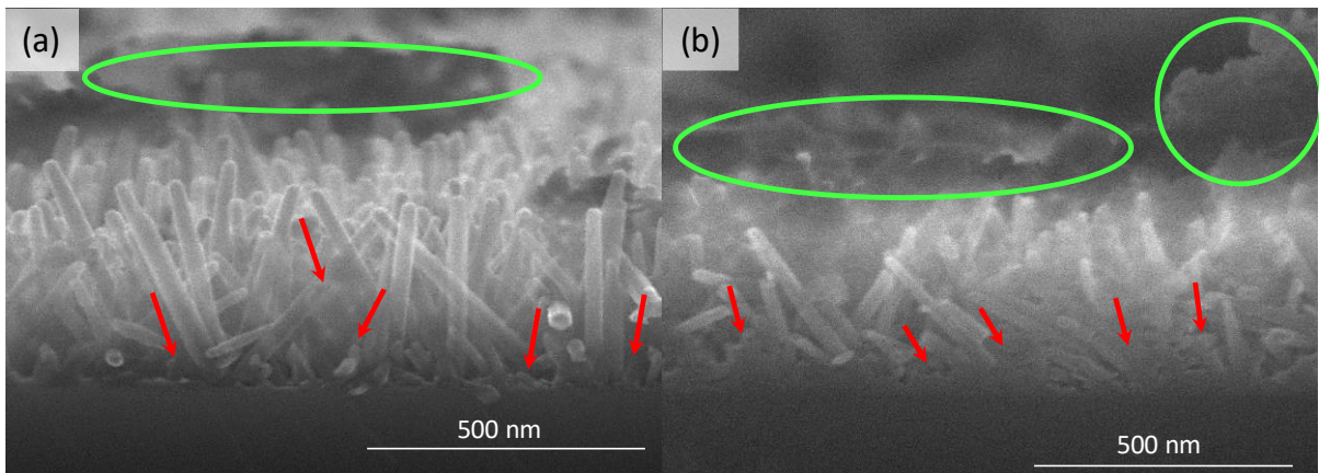
Figure 7 : Cross-sectional SEM images of ZnO/YAG:Ce composite coatings made with (a) 5 and (b) 20 impregnations of YAG:Ce NPs suspension. Red arrows indicate YAG:Ce NPs lying between ZnO NWs whereas green circles highlight the surface crust.
