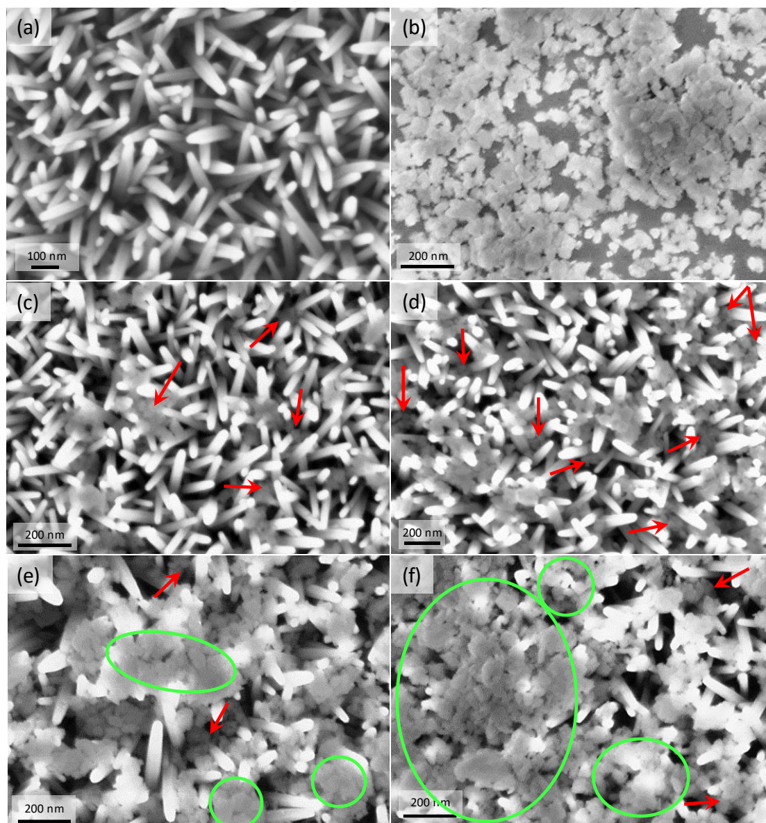
Figure 6 : SEM images of (a) ZnO NWs alone, (b) YAG:Ce alone (10 coatings of 20 g/L ground YAG:Ce suspension) and ZnO/YAG:Ce composite coatings made with (c) 5, (d) 10, (e) 15 and (f) 20 impregnations of YAG:Ce NPs suspension. In (c) to (f), red arrows indicate YAG:Ce NPs lying between ZnO NWs whereas green circles highlight the surface crust.
