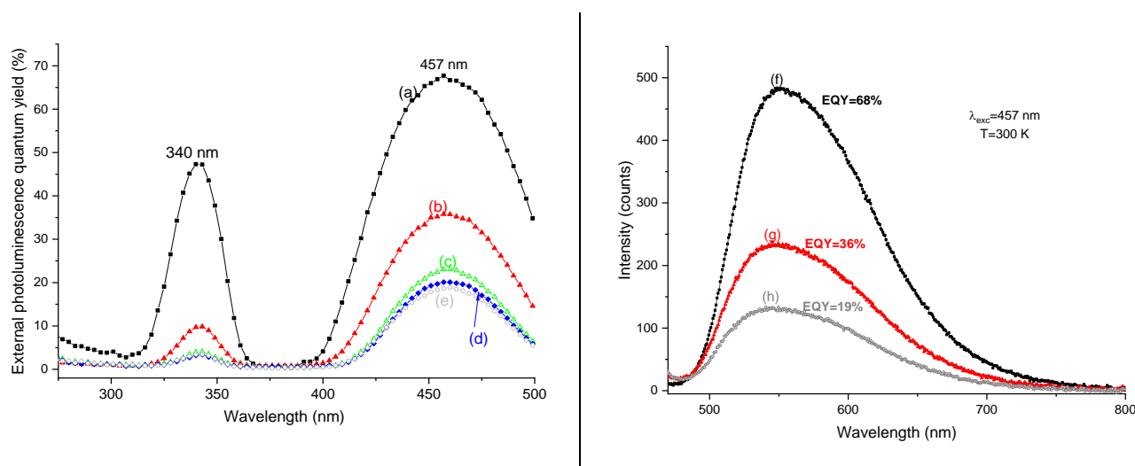
Figure 4 : Left - Evolution of the room temperature photoluminescence quantum yield versus excitation wavelength for commercial YAG:Ce before (a) and after grinding with various bead diameters / grinding durations: (b) 0.5 mm/30 min, (c) 0.1 mm/15 min, (d) 0.1 mm/30 min and (e) 0.1 mm/45 min. Right - Emission spectra of commercial YAG :Ce under
