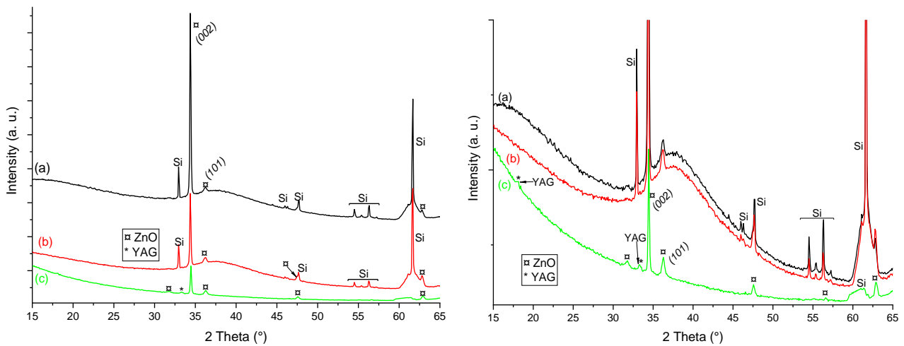
Figure 5 : Left: XRD patterns of (a) ZnO NWs alone and ZnO/YAG:Ce composite coatings made with (b) 5 and (c) 20 impregnations of YAG:Ce NPs suspension (Y offset has been used to better see the top of the most intense diffraction reflection) ; Right: Corresponding zoom-in (no Y offset used). Reflections of the Si substrate and YAG phase are indicated in the figure, and those of the ZnO component are indexed.
