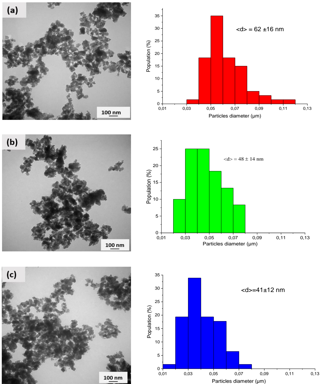
Figure 3 : TEM images and corresponding size distribution of powders ground with 0.1 mm beads during (a) 15, (b) 30 and (c) 45 min.
