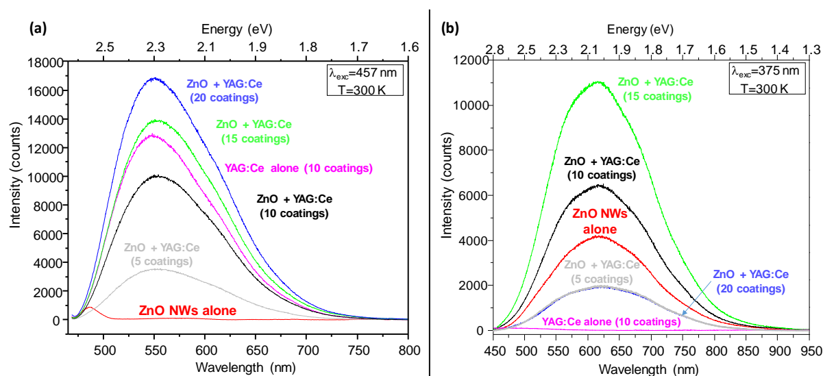
Figure 9 : Room temperature emission spectra of ZnO NWs alone, YAG:Ce alone (10 coatings of 20 g/L ground YAG:Ce suspension) and ZnO/YAG:Ce composite coatings made with 5 to 20 impregnations of 20 g/L YAG:Ce NPs suspension (a) under blue and (b) UV excitations.
