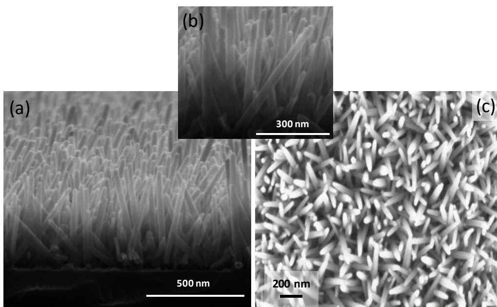
Figure 2 : (a), (b) Cross-sectional and (c) top SEM views of the as-grown ZnO NWs.
