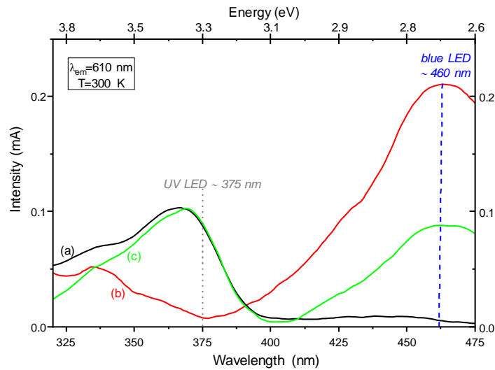
Figure 8 : Room temperature excitation spectra of (a) ZnO NWs alone, (b) YAG:Ce alone (10 coatings of 20 g/L ground YAG:Ce suspension) and (c) ZnO/YAG:Ce composite made with 10 impregnations of YAG:Ce NPs suspension.
