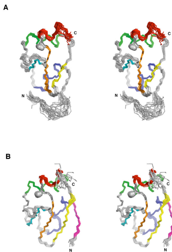
Figure 2. NMR ensembles of the E6 domain structures. Stereo views of the 20 lowest energy structures of E6N F47R (residues 1-71) ( A ) and E6C 4C/4S (residues 80-143) ( B ). Zinc atoms are represented as grey spheres. Figures of the molecular structures were made using PyMOL (DeLano). See also Figure S2.
