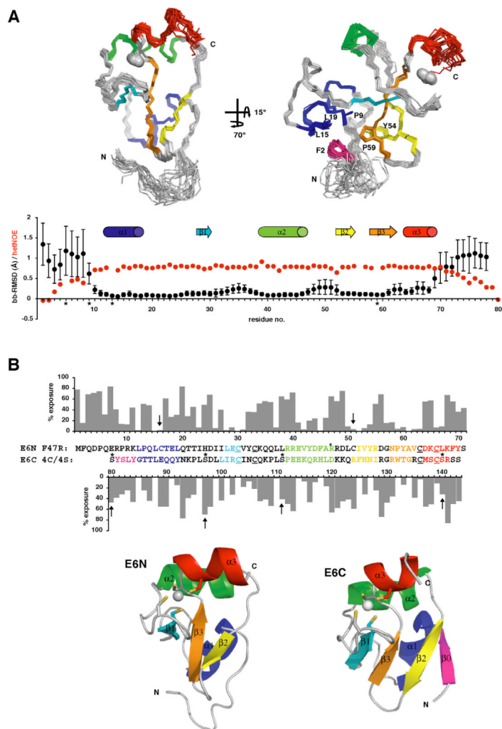
Figure 3. Structure and dynamic properties of the monomeric HPV16 E6 zinc-binding domains. (A) ( Upper panel ) Ensemble of the 20 lowest energy structures of E6N F47R. The right hand view shows the anchoring residue F2 and other hydrophobic core residues displaying NOE contacts with F2. ( Lower panel ) Heteronuclear NOE (red circles) and average pairwise backbone r.m.s. deviations (black circles) values for the E6N F47R domain. R.m.s. deviations have been calculated over five residue segments of the primary sequence for the 20 lowest energy NMR structures and error bars represent standard deviations of the mean. Black stars on the x-axis mark proline residues. (B) Structural homology of the E6N and E6C domains ( Upper panel ) Percentage of exposure to the solvent of residues in the lowest energy NMR structures of E6N F47R and E6C-4C/4S constructs. The y-axis of the E6C plot has been inverted for clarity. Numbers on the x-axis correspond to the wild-type HPV16 E6 sequence. The amino acid sequence of each domain is aligned with the x-axis and coloured to mark secondary structure elements. Zinc coordinating cysteines are underlined, while exposure values for non-conserved cysteines are indicated by arrows. Asterisks indicate sites of mutations. ( Lower panel ) Ribbon representations of the lowest energy NMR structures of the E6N F47R (left) and E6C 4C/4S (right) constructs. Zinc atoms and coordinating cysteine side-chains are displayed. See also Figure S3.
