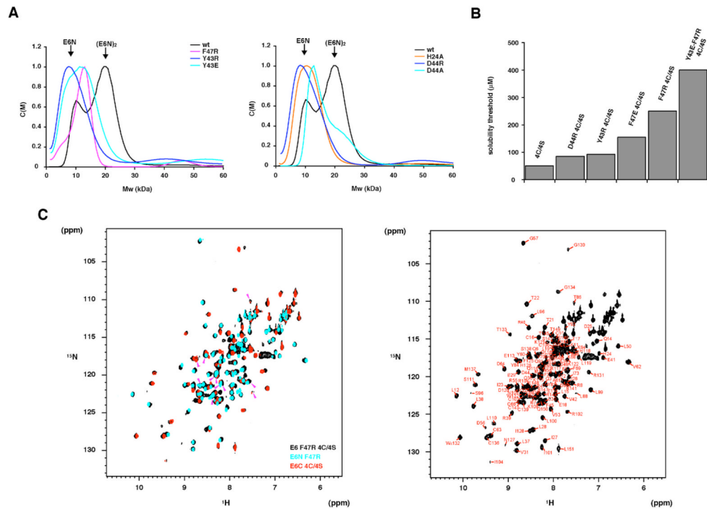
Figure 5. Mutations at the E6N homodimer interface enhance full-length E6 solubility. (A) Homodimer interface mutations have been introduced in the context of HPV16 E6N domain construct and the resulting samples have been analyzed by sedimentation velocity ultracentrifugation experiments. The profile of the wild-type domain is reported on each plot for clarity. (B) Concentrations thresholds of samples of full-length E6 mutants. Homodimer interface mutations have been introduced in the HPV16 E6 4C/4S construct. (C) ^1\text{H} , ^{15}\text{N} HSQC spectra of the E6 F47R 4C/4S construct. ( Left panel ) Superposition of spectra of E6 F47R 4C/4S (black), E6N F47R (cyan) and E6C 4C/4S (red) constructs. Magenta arrows indicate amide groups belonging to residues 1-10 and 80-90. ( Right panel ) Annotated ^1\text{H} , ^{15}\text{N} HSQC of E6 F47R 4C/4S. Assignments are shown in red. See also Figure S5.
