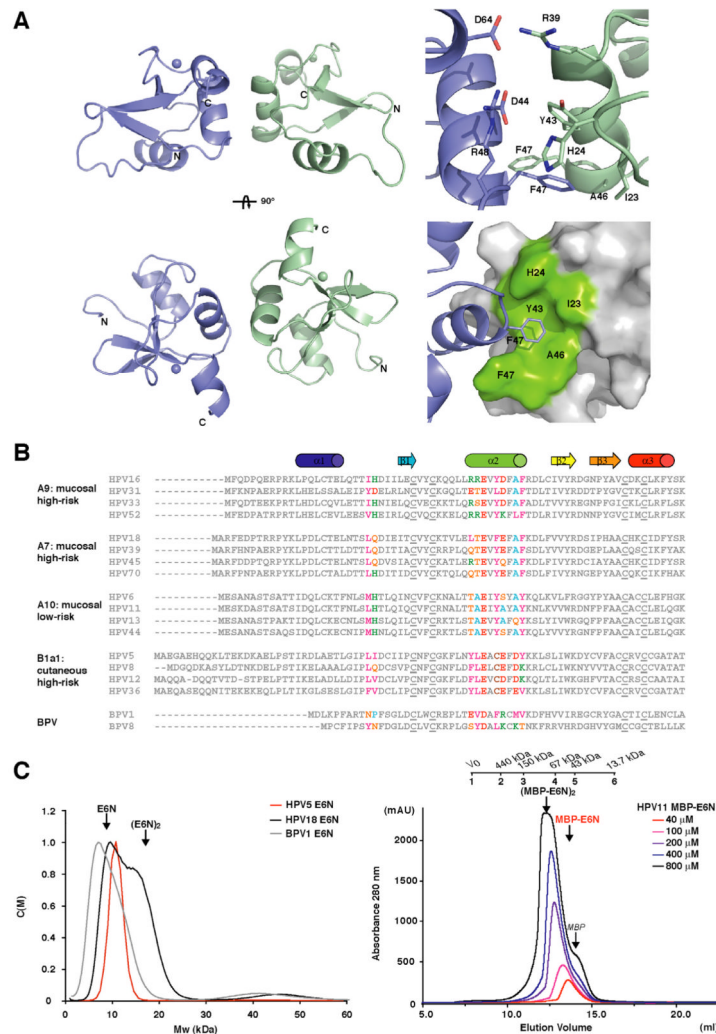
Figure 4. Model structure of the HPV16 E6N homodimer. (A) (Left panel) Ribbon representation of the lowest energy structure in cluster 1. (Right panel) Views of the homodimer interface. The top representation illustrates the side-chain orientation of interacting residues. The bottom representation illustrates the positioning of the aromatic ring F47 (violet) in the shallow hydrophobic pocket (green) within the opposing subunit. (B) Alignment of E6N sequences of representative strains from the “high-risk” mucosal HPV A9 and A7 groups, the low-risk mucosal A10 group, the “high-risk” cutaneous B1A1 group and two BPV strains. Residues reported to undergo the largest chemical shift variations in Figure 1D are coloured according to their physicochemical properties as follows: magenta, hydrophobic (W, F, Y, L, I, V, M); green, basic (K, R, H); red, acidic (E, D); orange, polar (Q, N, T, S); brown, cysteine (C); cyan, small (G, A, P). (C) (Left panel) Molecular weight distribution of wild-type HPV5, HPV18 and BPV1 E6N domain constructs derived from sedimentation velocity ultracentrifugation experiments. (Right panel) Analytical gel filtration chromatography analysis of affinity purified HPV11 MBP-E6N fusion construct. Samples were adjusted at the concentrations indicated and injected on a Superdex 200 10/30 column. The elution volumes of the monomeric (MBP-E6N, 55.2 kDa) and dimeric ((MBP-E6N) 2 , 110.4 kDa) species are indicated. The shoulder at 14.1 ml corresponds to MBP arising from residual proteolytic activity in the preparations. Molecular size markers are reported on top
