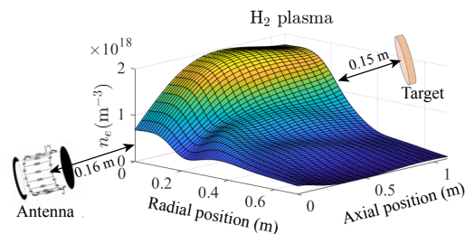
Figure 2. 3D cylindrically-symmetric interpolated profile of plasma density in the vessel measured with a two axis LP and calibrated with a 100 GHz heterodyne microwave interferometer. Measurements start 0.16 m from the near end of the antenna and stop 0.15 m before the target.
