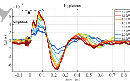
Figure 7. Typical photodetachment signals for a H 2 plasma. The laser strikes the LP tip at t = 0 s causing the overshoot whose amplitude is indicated by the arrow.
