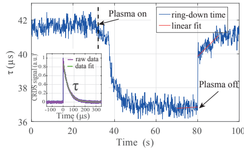
Figure 5. Ring-down time \tau before, during, and after a plasma discharge for a \text{H}_2 plasma and 5 kW RF power. The plasma discharge starts at t \cong 30 s and it is stabilized after a few seconds. Plasma is turned off at t = 80 s causing the jump of \tau due to the disappearance of \text{H}^- ions. The linear fit of \tau before and after the plasma off is used to accurately determine \tau at plasma off. The jump is used to evaluate the line-averaged \text{H}^- density. The inset shows a fit as used to calculate the ring-down time for each data point \tau .
