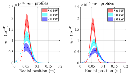
Figure 12. n_{H^-} and n_{D^-} radial profiles for different powers obtained using the relative negative ion profiles measured with laser photodetachment and calibrated with CRDS line-integrated measurements.
