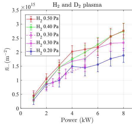
Figure 6. Line-integrated negative ion density as a function of RF power at different pressures for H 2 and D 2 plasmas, demonstrating the steady-state production of negative ions up to 8 kW of RF power.
