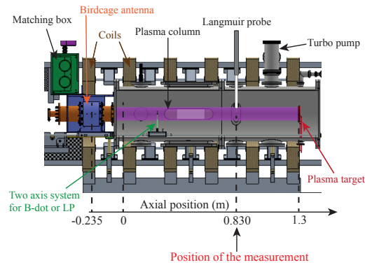
Figure 1. A cross section of the RAID plasma device along the axis. The cylindrical vacuum vessel of 1.4 m length and 0.4 m diameter is surrounded by six coils producing an axial magnetic field up to 800 G. The resonant birdcage antenna, placed on the left, produces a plasma column up to the target on the right.
