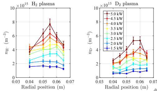
Figure 9. Radial profiles of negative ion density obtained with laser photodetachment and measuring the electron density via IV curves. These data are not calibrated with CRDS.
