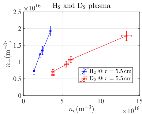
Figure 14. Negative ion density vs. electron density in hydrogen and deuterium plasmas.
