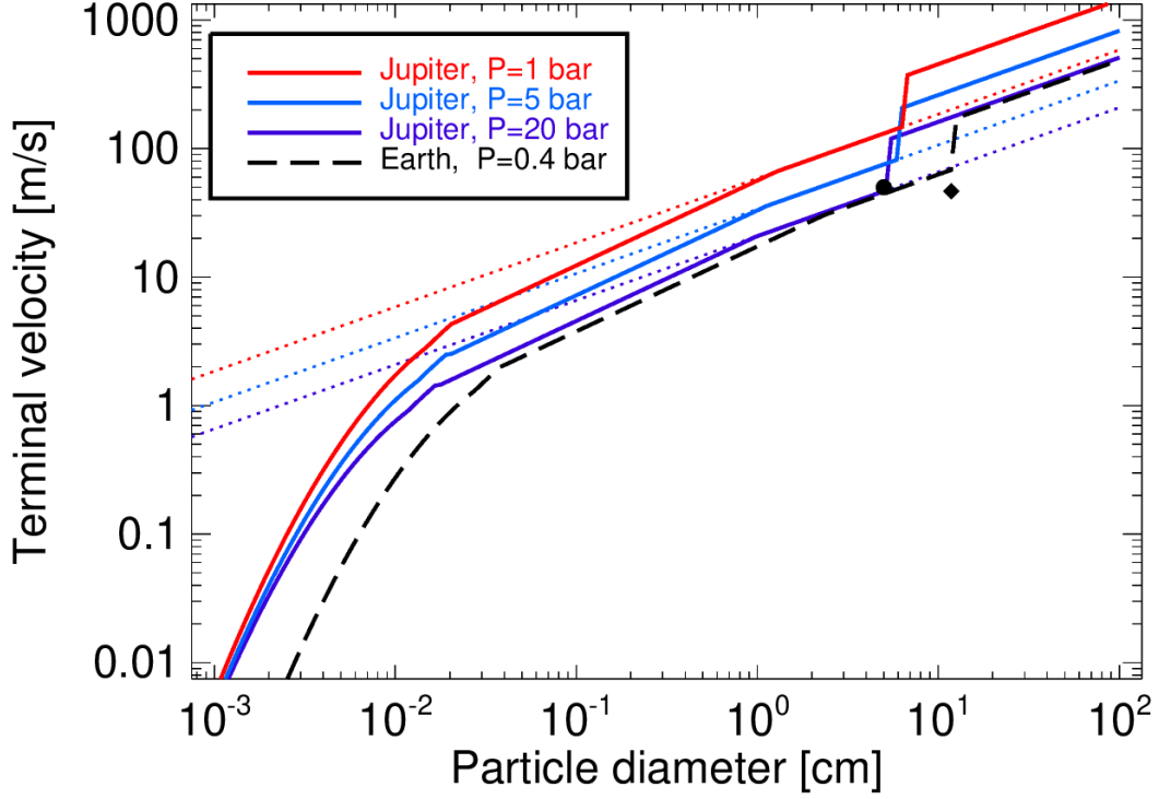
Figure 2. Terminal velocity of ice (or ammonia-ice) particles with diameters from 1 \mu\text{m} to 1\text{m} , for three pressure levels, 1, 5 and 20 bar inside Jupiter’s atmosphere. The plain lines correspond to the full formulation. The dotted lines are the result from assuming a constant drag C_d=0.6 , applicable to large Earth hailstones (Rasmussen & Heymsfield, 1987). For comparison the Earth case for a pressure of 400 mbar and a temperature of -20^\circ\text{C} is shown as a dashed line. Two examples for the Earth case are shown: The circle corresponds to 5cm hailstones observed in a particularly powerful storm which occurred in Oklahoma on 1976/05/29, with updrafts of \sim 50\text{ m/s} (Nelson, 1983). The diamond corresponds to a giant hailstone collected on 1970/09/03 also in Oklahoma, weighting 766 g, with 15.5 cm of longest dimension and 11.8 cm of effective diameter (Roos, 1972).
