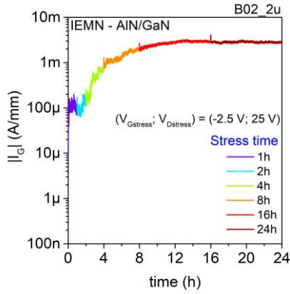
Fig - 17. Variation of gate current during 24h step-stress experiment carried out at (V_{GStress}, V_{DStress}) = (-2.5 V, 25 V) with the electrical parameters monitored at 1h, 2h, 4h, 8h, 16h and 24h of AlN/GaN HEMT
