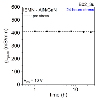
Fig - 16. g_{mpeak} at V_{DS} = 10 \text{ V} monitoring during 24h stress carried out at (V_{GStress}, V_{DStress}) = (-2 \text{ V}, 20 \text{ V}) of AlN/GaN HEMT
