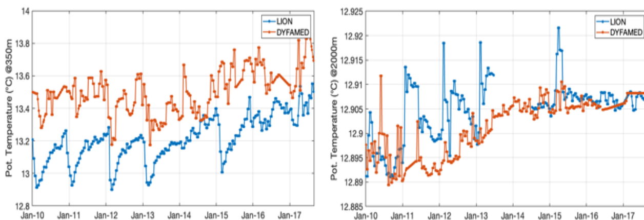
Fig. 3. Interpolated potential temperature data at depths of 350 meters (left) and 2,000 meters (right) from the LION and DYFAMED moorings (blue and red, respectively) from January 2010 to July 2017 (from EMSO).
