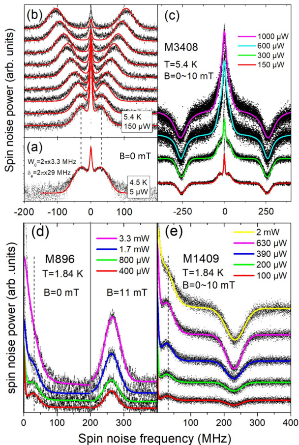
FIG. 2. Spin noise spectra obtained from three different samples and different detection configurations: (a,b,c) M3408 and heterodyne and self-homodyne detection; (d,e) M896, M1409 respectively and self-homodyne detection. (a) Zero magnetic field spin noise. (b) Series of noise spectra for increasing magnetic fields from 0 to 4 mT in steps of 0.5 mT. The red curves are fits of the data with Glazov’s model [24] ( W_0 is the hopping rate, and \delta_e represents the dispersion of the nuclear field distribution, see Sec. III B). (c,d,e) Series of noise spectra for different probe powers. The spectra in (c,e) are obtained by taking the difference between spectra measured at zero and non-zero magnetic field. The spectra in (d) are obtained either at zero magnetic field or in a field of 11 mT. In all panels the lines at zero magnetic field (close to zero frequency) are fitted with Glazov’s model, while the lines in non-zero magnetic field (at frequencies above typically 200 MHz) are fitted with gaussian, excepted at 150 and 300 \mu\text{W} in (c) where the lines are fitted with lorentzian. In (b,c,d,e) the curves are vertically offset for clarity.
