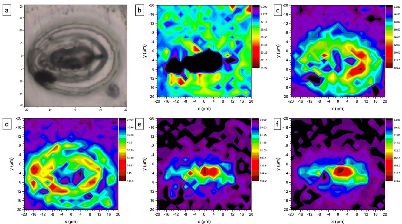
Fig. 3. a) Optical micrograph of the scanned area test and the variation of the intensity of the following peaks: b) \text{Mg}_{17}\text{Al}_{12} ( 700\text{--}900\text{ cm}^{-1} ), c) Mg ( 960\text{--}1000\text{ cm}^{-1} ), d) MgO ( 1030\text{--}1110\text{ cm}^{-1} ), e) H1 ( 4015\text{--}4135\text{ cm}^{-1} ), and f) H2 ( 4135\text{--}4255\text{ cm}^{-1} ).
