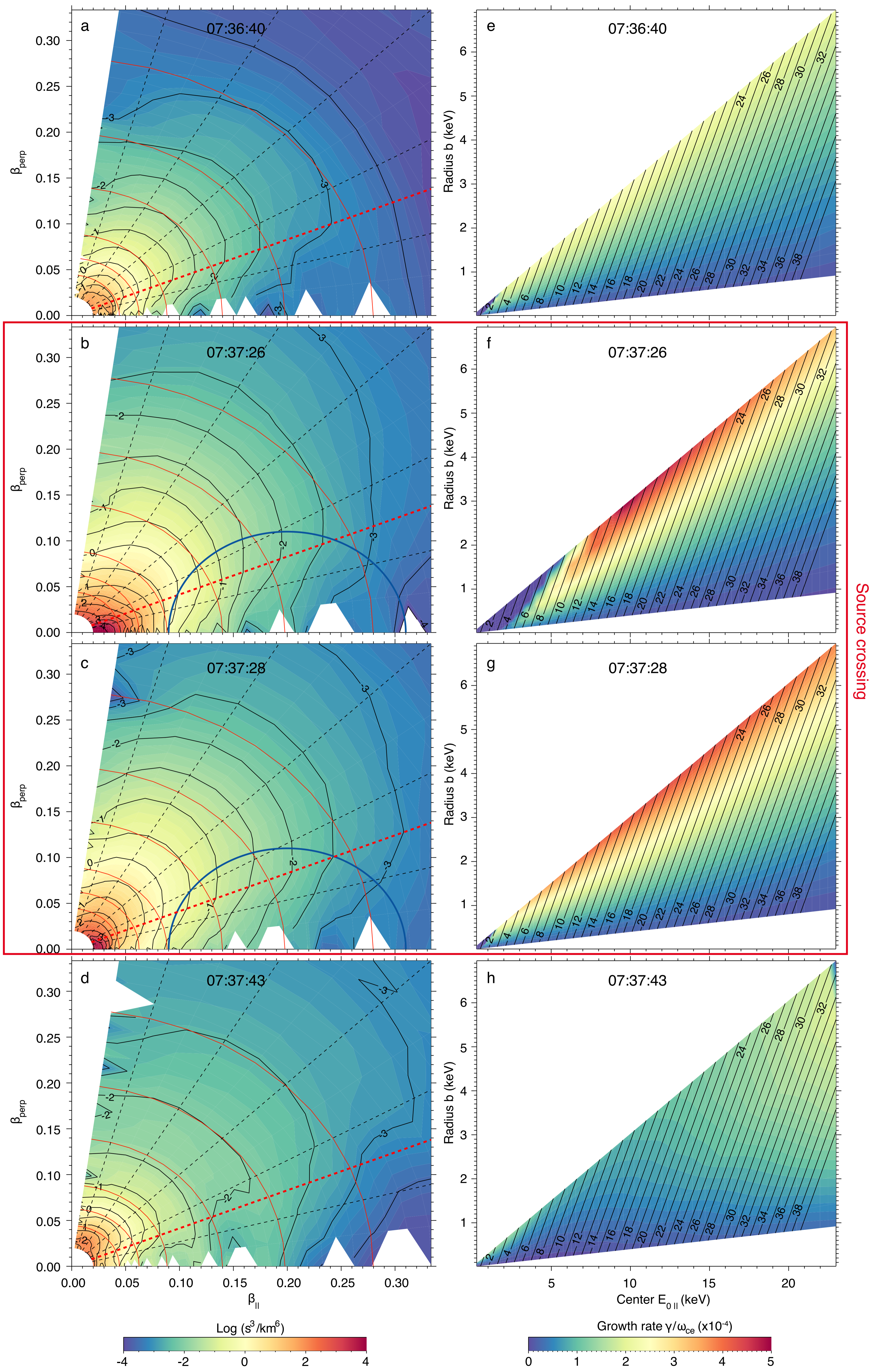
Grow rate \gamma/\omega_{ce} and \Delta\omega iso-contour along resonant circles
