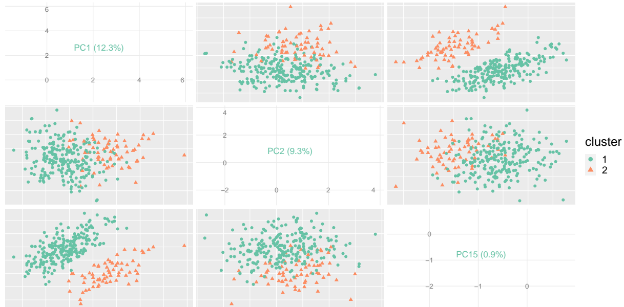
Figure 1: Chang (1983) data set with n = 300 observations projected on the 1st, 2nd and 15th principal components respectively. Colors and shapes indicate the true cluster membership. We see that the last principal component contains important discriminative information in terms of clustering, while the second principal component is not suited for the task.
