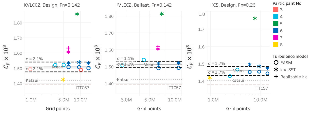
Fig. 14. Full scale CFD simulations. Computed frictional coefficient, C_F , for KVLCC2 hull in design loading condition at F_n = 0.142 (left), KVLCC2 in ballast loading condition F_n = 0.142 (center) and KCS hull in design loading condition at F_n = 0.26 (right).
