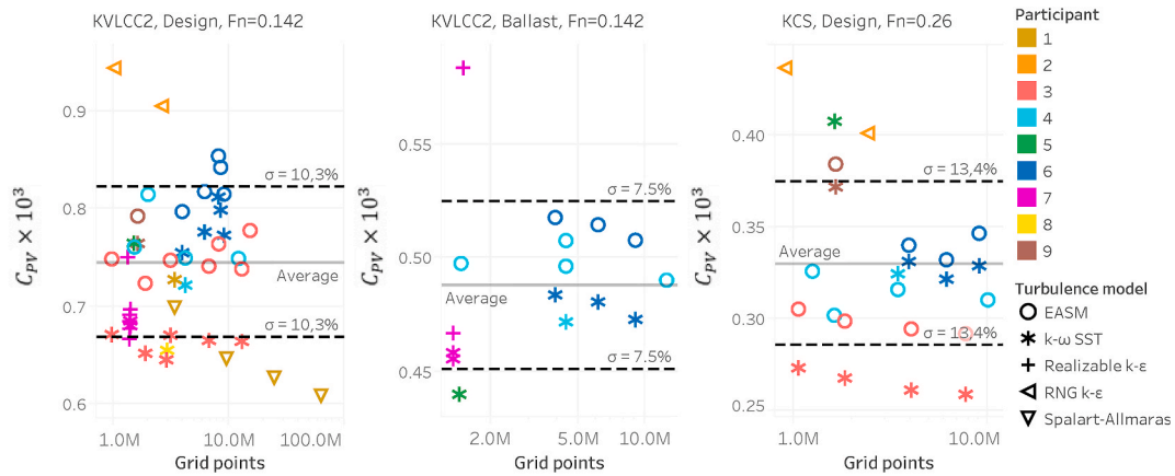
Fig. 8. Viscous pressure coefficient, C_{pv} , in model scale for KVLC2 hull in design loading condition at Fn=0.142 (left), KVLC2 in ballast loading condition Fn=0.142 (center) and KCS hull in design loading condition at Fn=0.26 (right).
