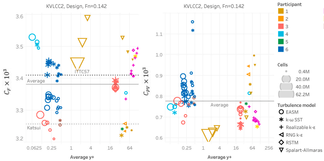
Fig. 9. C_f (left) and C_{pv} (right) in model scale for KVLC2 hull in design loading condition at Fn=0.142 against mean y^+ . y^+ < 1 : wall resolved, y^+ > 1 : wall function.
