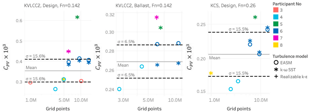
Fig. 15. Full scale CFD simulations. Computed viscous pressure coefficient, C_{PV} , for KVLCC2 hull in design loading condition at F_n = 0.142 (left), KVLCC2 in ballast loading condition F_n = 0.142 (center) and KCS hull in design loading condition at F_n = 0.26 (right).
