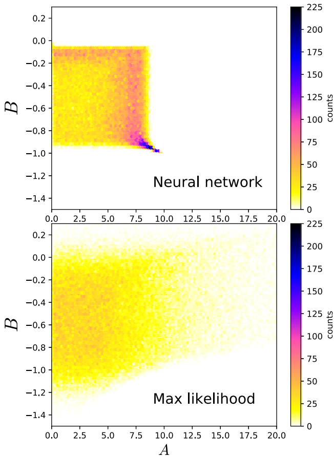
Figure 3. We take 100,000 power spectra from the AstroNone set with k_{\max} = 0.05 h \text{ Mpc}^{-1} , and predict the values of the cosmological parameters A and B for each using the neural network (top panel) and the maximum likelihood (bottom panel) methods. Cells are color coded according to the number of points within each cell. The neural network always predicts values of A and B within the range of [0.1, 10] and [-1, 0] , while the least squares method output values in a much wider range: A \in [0, 425] , B \in [-1.7, 0.8] . This shows how the neural network has learned the priors on the distribution of the parameters and never predicts values outside that range. This is the reason why the variance of the neural network is lower than the one of the maximum likelihood method.
