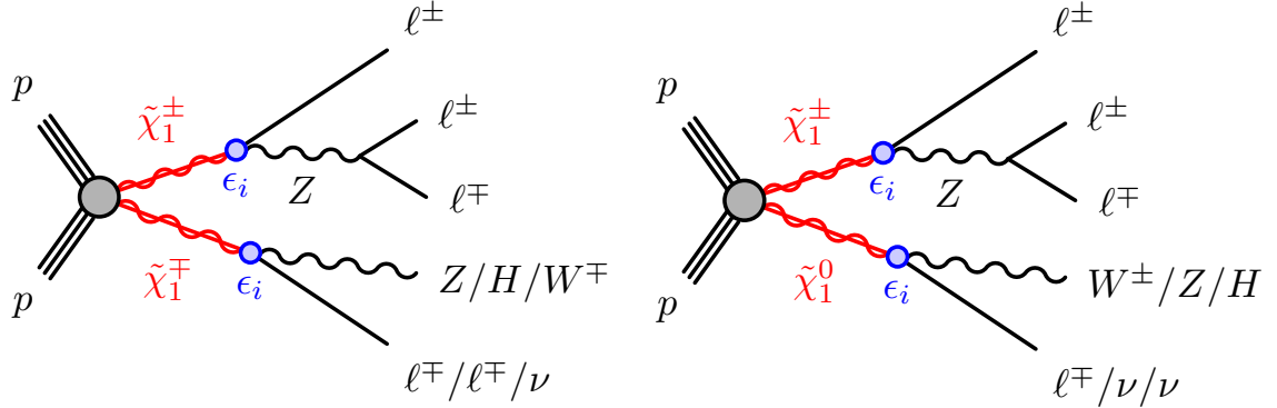
Figure 1: Diagrams of (left) \tilde{\chi}_1^\pm \tilde{\chi}_1^\mp and (right) \tilde{\chi}_1^\pm \tilde{\chi}_1^0 production with at least one \tilde{\chi}_1^\pm \rightarrow Z\ell \rightarrow \ell\ell\ell decay. The R -parity-violating coupling \epsilon_i allows prompt \tilde{\chi}_1^\pm decays into Z\ell , H\ell , or W\nu and prompt \tilde{\chi}_1^0 decays into W\ell , Z\nu , or H\nu .
