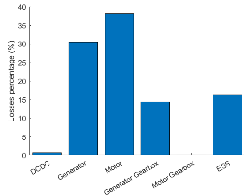
Figure 5: Losses percentage overview of the reference design (non-optimized)
