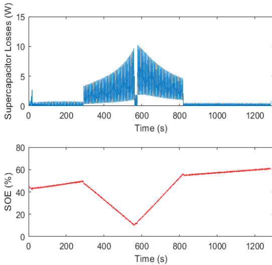
Figure 7: SOE and ESS losses for the hilly trip
