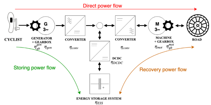
Figure 1: Series Hybrid Bike architecture and associated efficiencies
