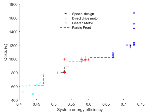
Figure 9: optimization result for a flat land drive
