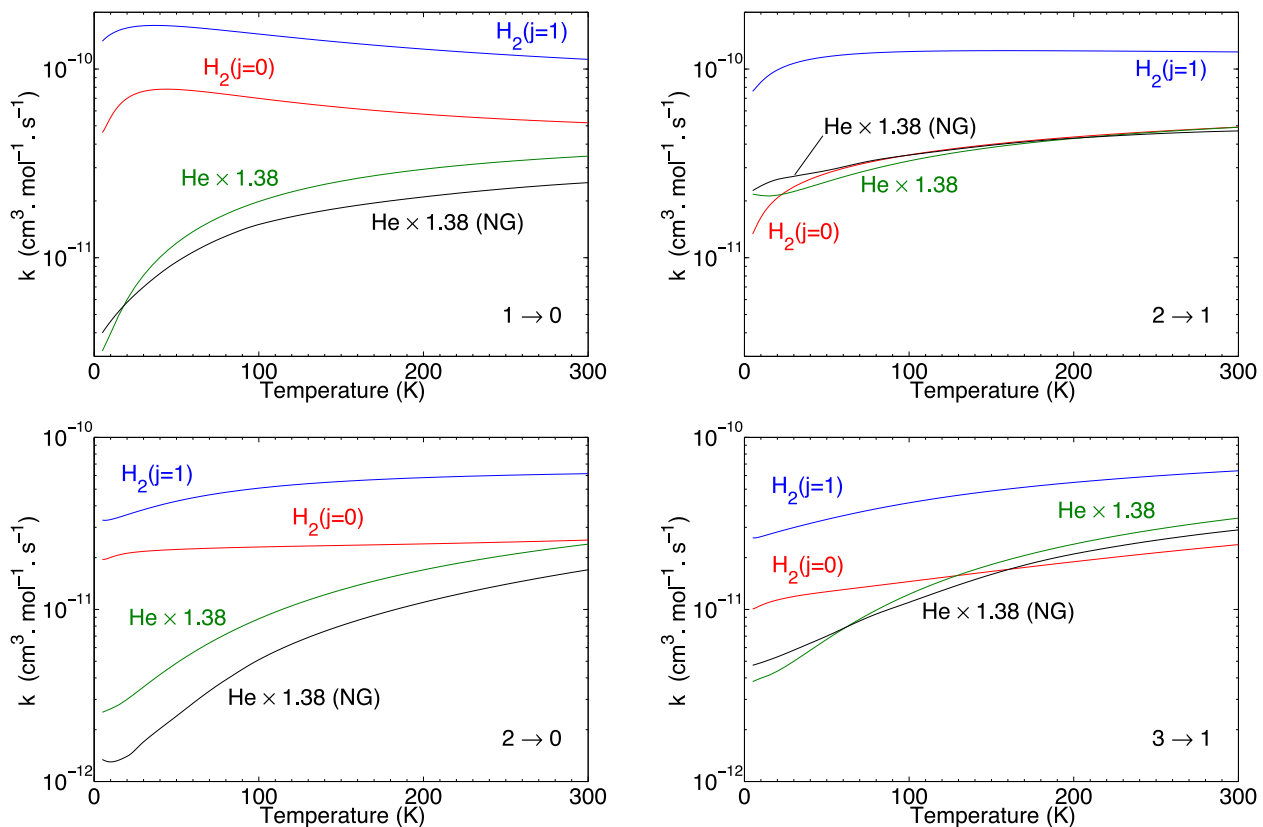
Figure 4. Rotational de-excitation rate coefficients of HCl by para- \text{H}_2 ( j_2 = 0 ) (red lines), by ortho- \text{H}_2 ( j_2 = 1 ) (blue lines) and by He scaled by 1.38 (Lanza & Lique 2012 : green lines and NG: black lines).
