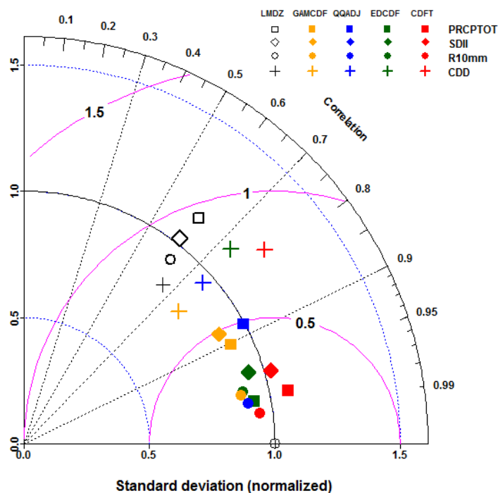
Figure 4. Taylor diagram showing the performance in reproducing the spatial pattern of four rainfall indices (PRCPTOT, SDII, R10mm and CDD) during the validation period (1986-2005) before (black) and after corrections using GamCDF (orange), QQadj (blue), EDCDF (green) and CDF-t (red).
