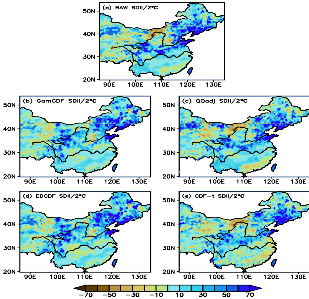
Figure S2. As in Fig. S1, but for SDII.
