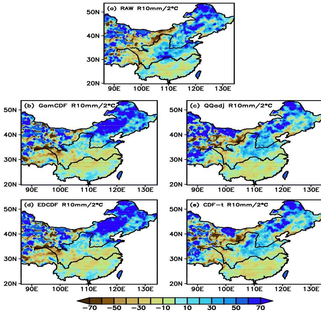
Figure S3. As in Fig. S1, but for R10mm.
