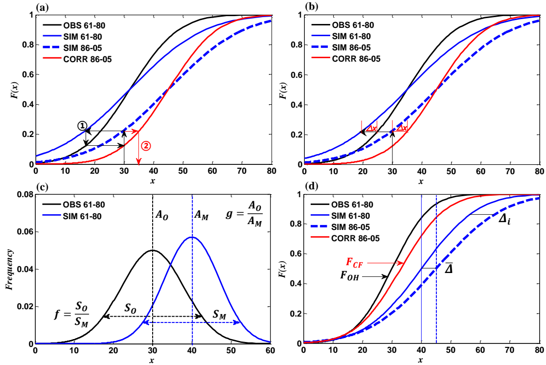
Figure 1. Schematic illustration of Transform Cumulative Distribution Function Method (a), Equidistant Cumulative Distribution Function Matching Method (b) and Quantile-Quantile Adjustment (c, d). CDFs of daily rainfall are shown for the observed control (OBS 61-80, black solid curve), raw control (SIM 61-80, blue solid curve), raw validation (SIM 86-05, blue dotted curve) and corrected (CORR 86-05, red solid curve) data. Black (red) arrows denote the segment ① (②) for (a). \Delta x represents the difference between the observation and the simulation at a specific percentile for (b). Black and blue dotted vertical lines represent mean values for observations and simulations over the historical period for (c). Blue solid and dotted vertical lines denote mean values for raw and future simulated period for (d).
