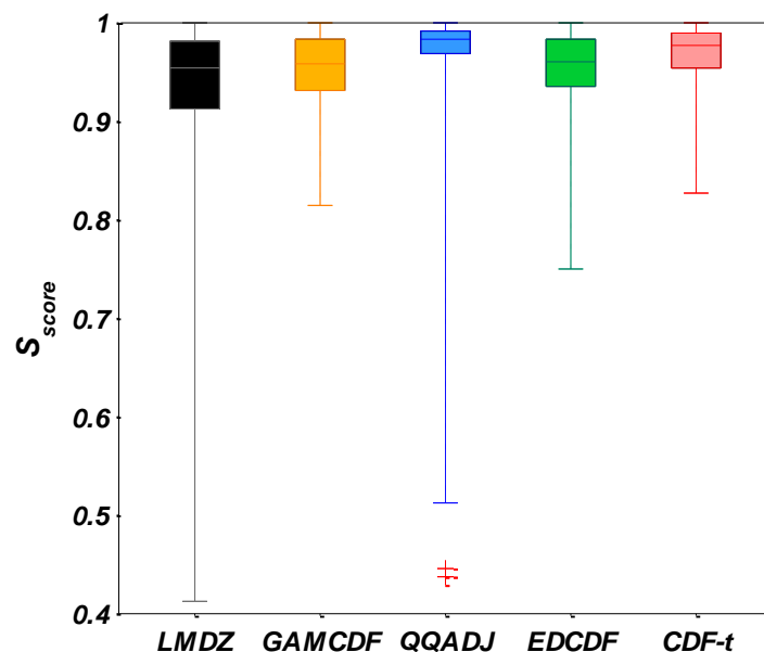
Figure 3. Box-and-whisker plot (The five-number summary is the minimum, first quartile, median, third quartile, and maximum) of S_{score} measuring PDFs of daily precipitations during the validation period (1986-2005) at all grid points over China before (black) and after corrections of GamCDF (orange), QQadj (blue), EDCDF (green) and CDF-t (red).
