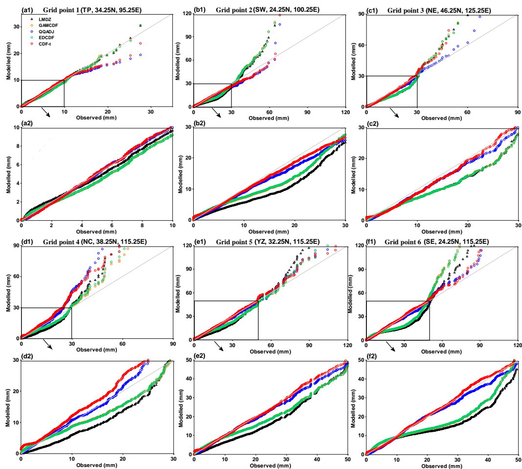
Figure 2. Quantile-Quantile plots of simulated daily precipitation during the validation period (1986-2005) in multi-model ensemble of RCMs (black), GamCDF (orange), QQadj (blue), EDCDF (green) and CDF-t (red) after correction, and observations at six grid points locating in Tibet Plateau (34.25°N, 95.25°E, a1, a2), Southwestern (24.25°N, 100.25°E, b1, b2), Northeastern, Northern (46.25°N, 125.25°E, c1, c2), Northern (38.25°N, 115.25°E, d1, d2), middle and low reaches of the Yangtze River (32.25°N, 115.25°E, e1, e2) and Southern region (24.25°N, 115.25°E, f1, f2), respectively.
