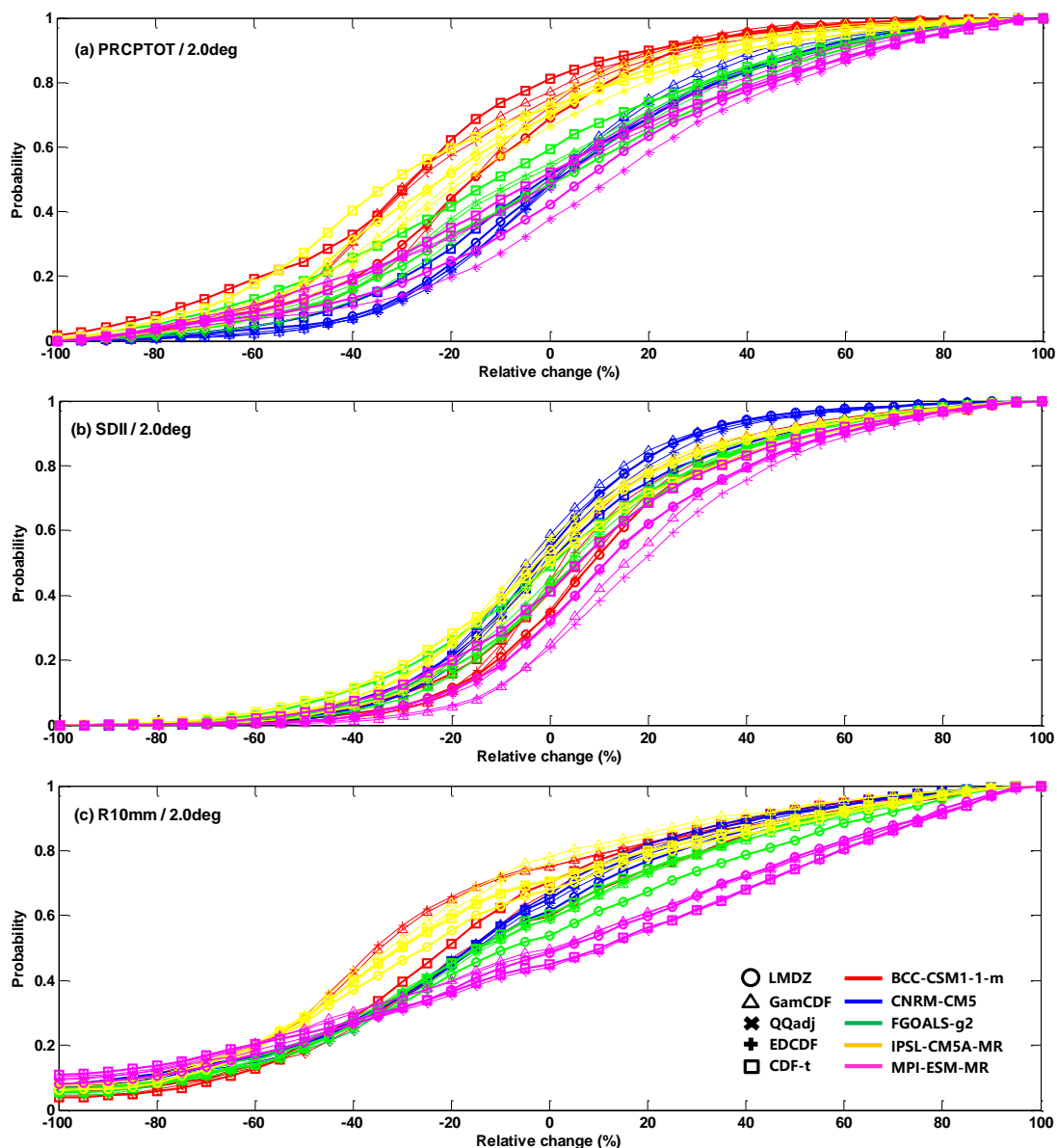
Figure 6. Cumulative probability Distribution Functions (CDFs) constructed over whole China for values of relative changes (in %) in PRCPTOT (a), SDII (b) and R10mm (c) under the 2.0-degree warming target. There are 25 curves in the first three panels, with five RCM simulations shown in different colors, and the original (LMDZ) and four bias correction results shown in different symbols.
