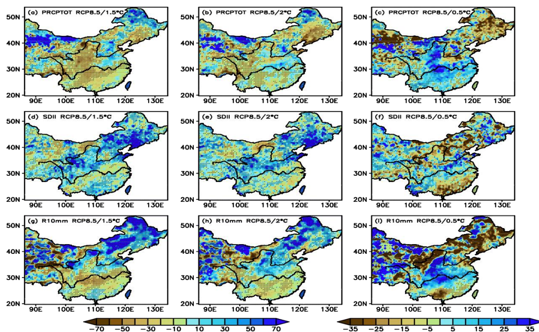
Figure 5. Relative changes in PRCPTOT (a, b, c), SDII (d, e, f) and R10mm (g, h, i) based on CDF-t under the global warming of 1.5°C (first column), 2°C (second column) and the half-degree addition (third column), relative to 1986-2005 (unit: %). The areas which all four methods agree with the sign of change in the raw RCM are indicated by dots.
