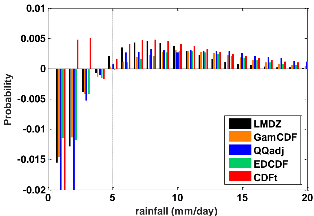
Figure S4. Difference of frequency between present and future daily precipitation under the 2.0°C target for the original and bias-adjusted RCM for an exemplary RCM simulation with LMDZ4 driven by BCC-CSM1-1-m.
