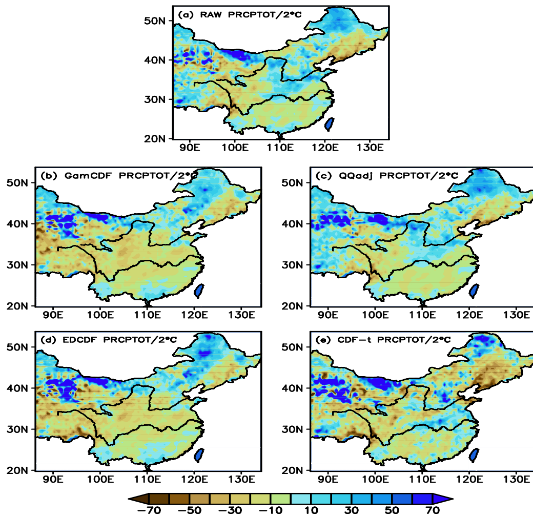
Figure S1. Relative changes (unit: %) in PRCPTOT from the raw RCMs (a), GamCDF (b), QQadj (c), EDCDF (d) and CDF-t (e) under the global warming of 2°C, relative to 1986-2005.
