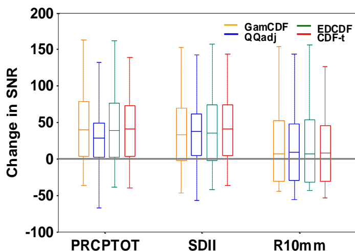
Figure 7. Boxplot showing relative changes (%) of the signal-to-noise ratio for PRCPTOT, SDII and R10mm using GamCDF (yellow), QQadj (blue), EDCDF (green) and CDF-t (red) compared with the raw RCMs at 2 degree warming target. The upper and lower limits of the box indicate the 75th and 25th percentiles among all grid points over the study area; the horizontal line inside the box indicates the 50th percentile (median); and the whiskers show the range among all grid points.
