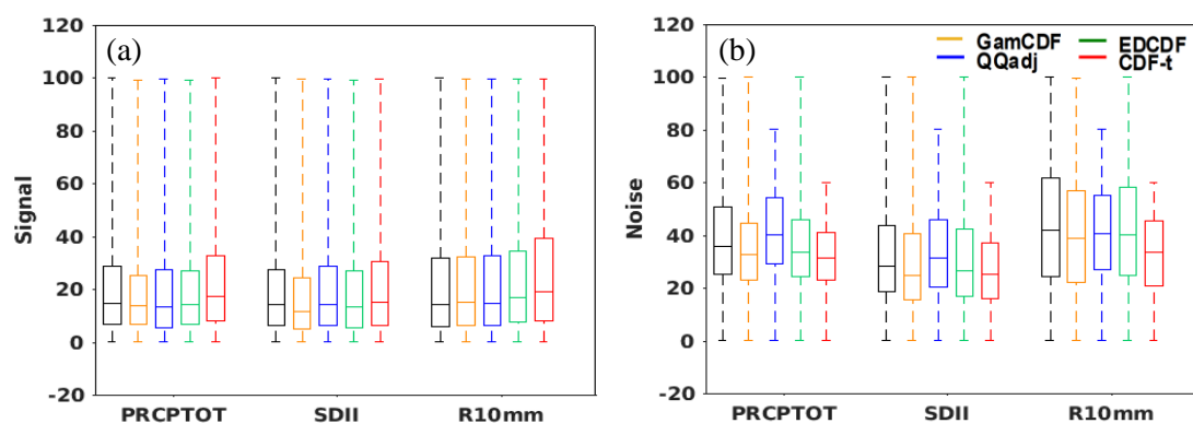
Figure S5. Signal (a) and noise (b) for PRCPTOT, SDII and R10mm before (black) and after corrections using GamCDF (yellow), QQadj (blue), EDCDF (green) and CDF-t (red) at 2 degree warming target. It's noted that the average and standard deviation of R10mm is 0 on the Northwestern region (NWR) due to the small precipitation. This causes that no SNR over the NWR is included in the Fig. 7.
