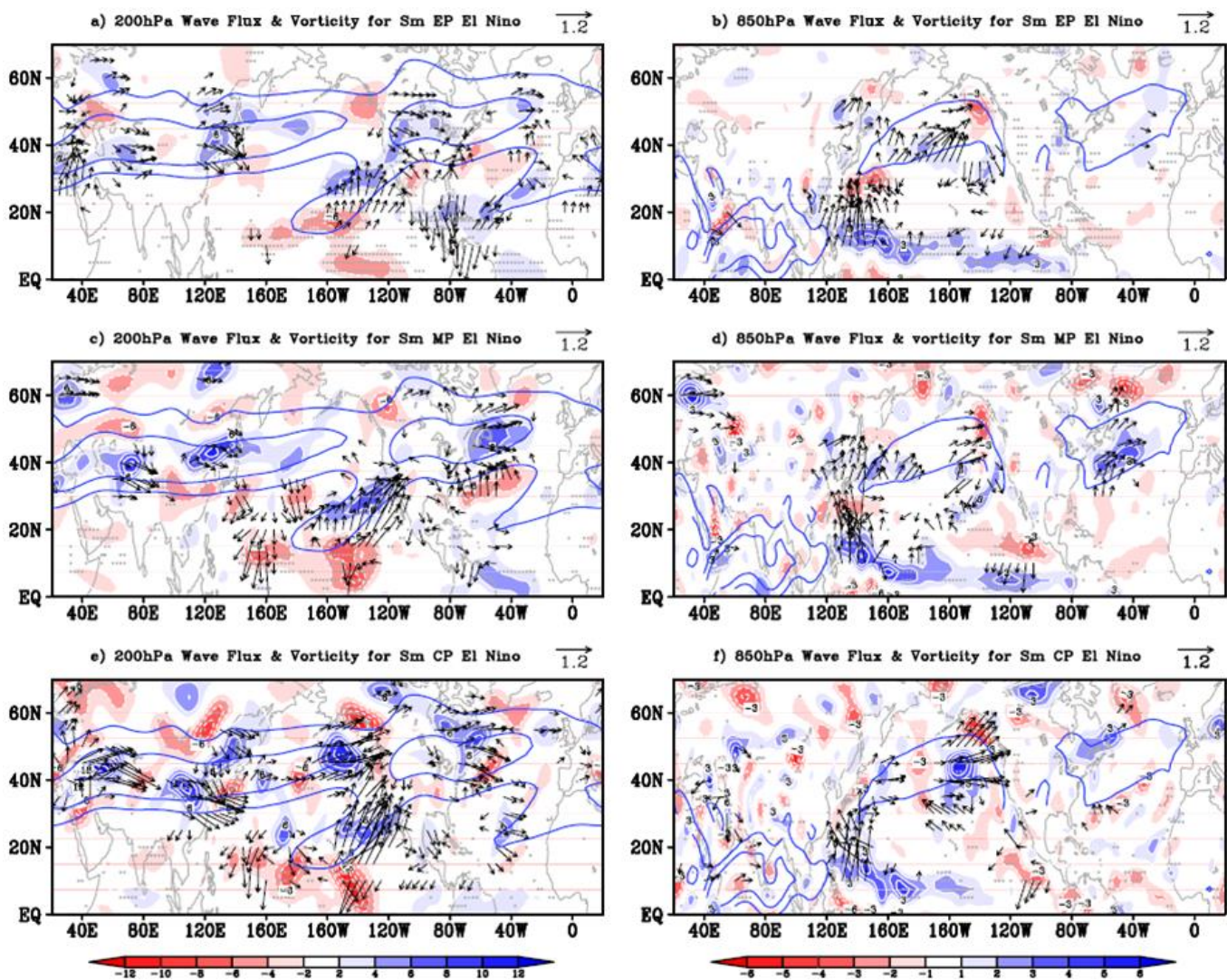
Figure 7 Composites of vorticity (shading, unit: s^{-1} ) and wave activity flux (vector, unit: m^2/s^2 ) at 200hPa (left panel) and 850hPa (right panel) in association with the different types of summer El Niño. From top to bottom are summer EP, MP and CP El Niño respectively. Contour intervals of the vorticity are 2 \times 10^{-6} s^{-1} at 200hPa and 1 \times 10^{-6} s^{-1} at 850hPa. Small values of the wave activity flux with magnitude less than 0.2 m^2/s^2 are omitted. The superimposed blue contours denote the climatological westerly wind, with speed 10, 20 m/s at 200 hPa and 5, 10 m/s at 850 hPa. The gray dots indicate the 90% confidence level.
