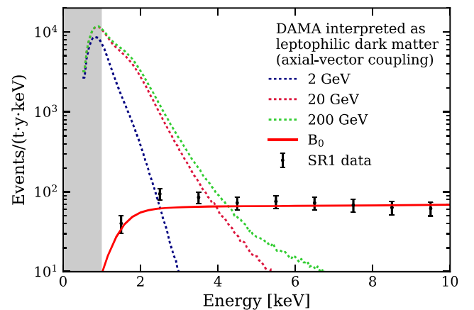
FIG. 14. Comparison between DAMA expected signals and XENON1T data (signal plus background). Dotted lines represent the expected signal spectra of selected masses in the XENON1T detector if the DAMA modulated signals are interpreted as WIMPs scattering on electrons through axial-vector interactions. XENON1T data are indicated by black points and the background model B_0 is illustrated by the red line. The right bound of the shaded region shows the threshold in this analysis.
