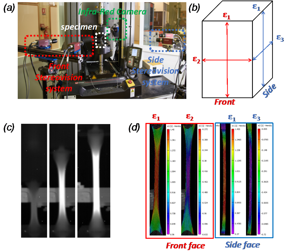
Figure 2. (a) Experimental Digital Image Correlation (DIC) set-up based on two independent stereo-vision systems to measure simultaneously strain fields on front and side surfaces of specimen, (b) Schematic representation of the front and side faces of the specimen with directions of the principal strain \epsilon_1 on front and side face, \epsilon_2 on front face and \epsilon_3 on side face. \epsilon_1 is calculated as the average value obtained on front and side surfaces, (c) traces of self-heating (in white) measured on the specimen surface at various deformation, (d) longitudinal and transverse strain fields analysed on front and side faces of the specimen for a given macroscopic deformation.
