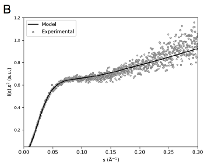
Figure S1. SAXS data and analysis of TIF2 NRID . A) Semi-logarithmic representation of the SAXS intensity versus momentum transfer s (open circles) and the averaged back-calculated curve derived from the final ensemble (2,000 conformers) that best explains the experimental RDCs (black curve) ( \chi^2 = 1.38 ). The bottom panel shows the residual of the fitting to the experiment. B) Kratky representation of the data show in A.
