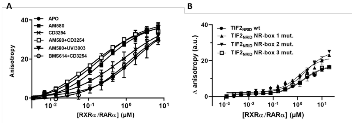
Figure S7 related to Figure 3 . A) Titration curves of FITC-labelled TIF2 NRID by RXR/RAR in the absence of ligand (Apo) or in the presence of an excess of RAR agonist (AM580), RXR agonist (CD3254), or combination of ligands including RAR antagonist (BMS614) and RXR antagonist (UVI3003). B) Titration of Alexa-labelled TIF2 NRID wt or mutant for each NR-box by RXR/RAR in the absence of ligand.
