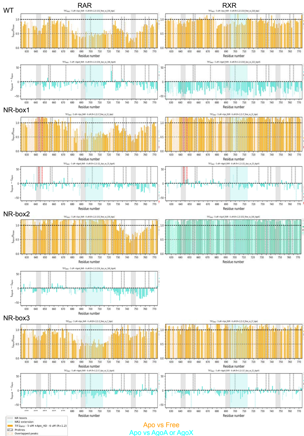
Figure S8 related to Figure 4 and 5 . Interaction of WT and LLxxAA mutated TIF2 NRID with apo and liganded RXR or RAR LBDs. Relative peak intensity ratios I_{Complex}/I_{TIF2NRID} and differential intensity I_{liganded\ complex} - I_{apo\ complex} for A) WT TIF2 NRID B) NR-box1 mutant C) NR-box 2 mutant C) NR-box3 mutant in complex with RAR (left column) or RXR (right column). Grey highlighted boxes indicate NR-boxes. Hashed bars correspond to prolines or ambiguous and overlapped peaks.
