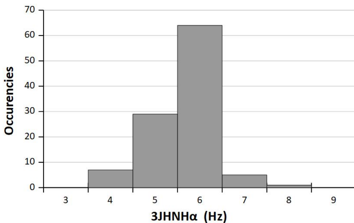
Figure S5. Histograms of the homonuclear ^3J_{\text{HNH}\alpha} coupling constants (in hertz) measured for TIF2 NRID . Values of 6-7 Hz indicate fast conformational averaging that is characteristic of random coil, while values below or above indicate helical or \beta -strand propensity, respectively. 65% of the measured values are in the range of 6-8 Hz.
