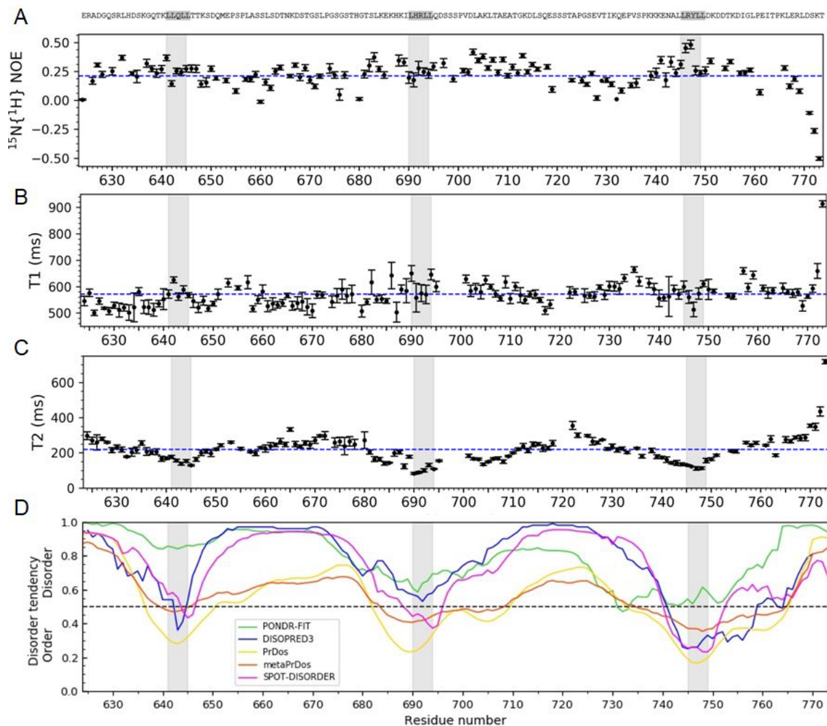
Figure S6. Related to Figure 2E . Backbone dynamics of TIF2 NRID per residue A) heteronuclear ^1\text{H} - ^{15}\text{N} NOE, B) ^{15}\text{N} - T_1 longitudinal, C) ^{15}\text{N} - T_2 transverse relaxation times and. Blue dashed lines represent the average values. All experiments were recorded at 10°C and at pH 6.8 with a 700 MHz spectrometer using 200 \mu\text{M} of protein in the NMR buffer. Disorder predictions D) from Figure 2 were added for easier interpretation of the data. Boxes highlighted in grey indicate NR Boxes (LxxLL motifs). Values and errors were calculated using Sparky. Proline, superimposed and ambiguous assigned residues were excluded from the analysis.
