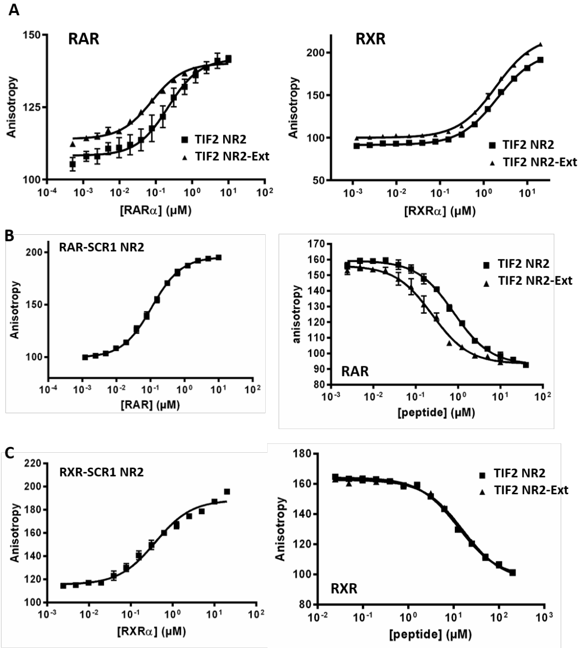
Figure S10 related to Figure 6 . A ) Titration curves of Alexa-labeled TIF2 NR2 and TIF2 NR2-Ext by RAR and RXR LBDs in the presence of AM580 (RAR agonist) and CD3254 (RXR agonist), respectively. B ) Direct titration of FITC-labeled SCR1 NR2 peptide by RAR LBD in the presence of the RAR agonist AM580 (left) and competition curves at 0.5 \mu\text{M} of RAR LBD of SCR1 NR2 by unlabeled TIF2 NR2 and TIF2 NR2-Ext peptides (right) in the presence of AM580. C ) Direct titration of FITC-labeled SCR1 NR2 peptide by RXR LBD in the presence of the RXR agonist LG100268 (left) and competition curves at 5 \mu\text{M} of RXR LBD of SCR1 NR2 by unlabeled TIF2 NR2 and TIF2 NR2-Ext peptides (right) in the presence of LG100268.
