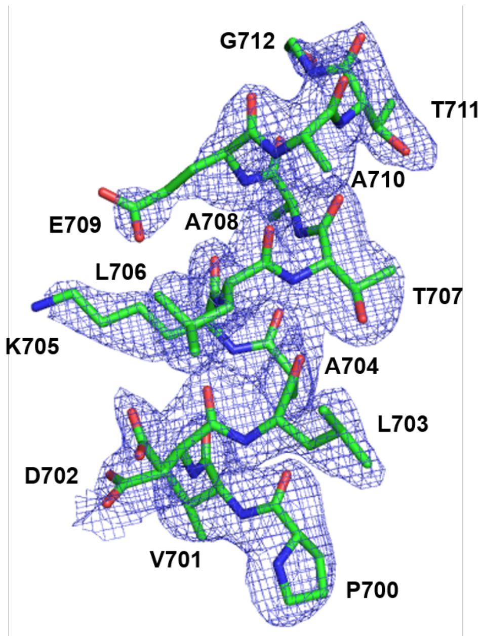
Figure S9 , related to Figure 6 . Helix \alpha 2 of TIF2 NR2-Ext peptide modelled into the difference density of the RAR LBD/TIF2 NR2-Ext crystal structure. Shown is an unbiased omit Polder map contoured at 2.5\sigma , with model bias reduction and exclusion of solvent density.
