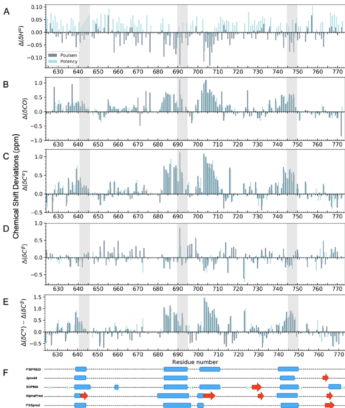
Figure S4. Related to Figure 2D . Secondary structure of TIF2 NRID from backbone secondary chemical shift analysis per residue A) H^\alpha B) CO C) C^\alpha and D) C^\beta chemical shift deviations from their random coil values obtained from the web servers: Poulsen IDP/IUP random coil chemical shifts (grey) and POTENCI (turquoise). E) Difference between C^\alpha and C^\beta secondary chemical shifts. A positive (negative) deviation of ^{13}C_\alpha and CO chemical shifts from their corresponding random coil values is an indication of \alpha -helical ( \beta -sheet) structure and vice versa for ^{13}C_\beta , ^1H_\alpha , ^{15}N and ^1HN . For H_\alpha nuclei, a large difference between values from the two databases is observed as already mentioned before by both authors (Kjaergaard et al., 2011; Kjaergaard and Poulsen, 2011; Nielsen and Mulder, 2018) F) Secondary structure predictions from Figure 2B were added for an easier interpretation of the data. Grey boxes indicate NR Boxes (LxxLL motifs). Prolines, superimposed and ambiguous assigned residues were excluded from the analysis.
