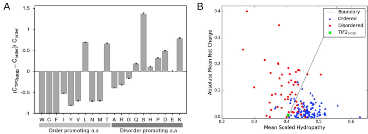
Figure S2. Related to Figure 1. A) Amino acid compositional analysis from Composition profiler server ( http://www.cprofler.org/ ). Amino acids are divided into order-promoting (hydrophobic and uncharged amino acids) and disorder-promoting (polar amino acids) categories. TIF2 NRID is compared to the reference value of the average amino acid frequencies of the PDB database. Positive bars correspond to residues found more in TIF2 NRID than in ordered proteins, whereas negative bars show residues that are depleted in TIF2 NRID . B) Uversky plot (mean scaled hydropathy vs mean net charge) as a predictor of disordered protein structure. A set of 54 completely disordered proteins, and 105 completely ordered proteins are shown as red circles and blue triangles, respectively. The solid line represents a boundary separating ordered and disordered proteins and is empirically defined by the equation: Hydropathy = (net\ charge + 1.151) / 2.785 . The green square corresponds to TIF2 NRID . Plot generated using PONDR ( http://www.pondr.com/ ).
