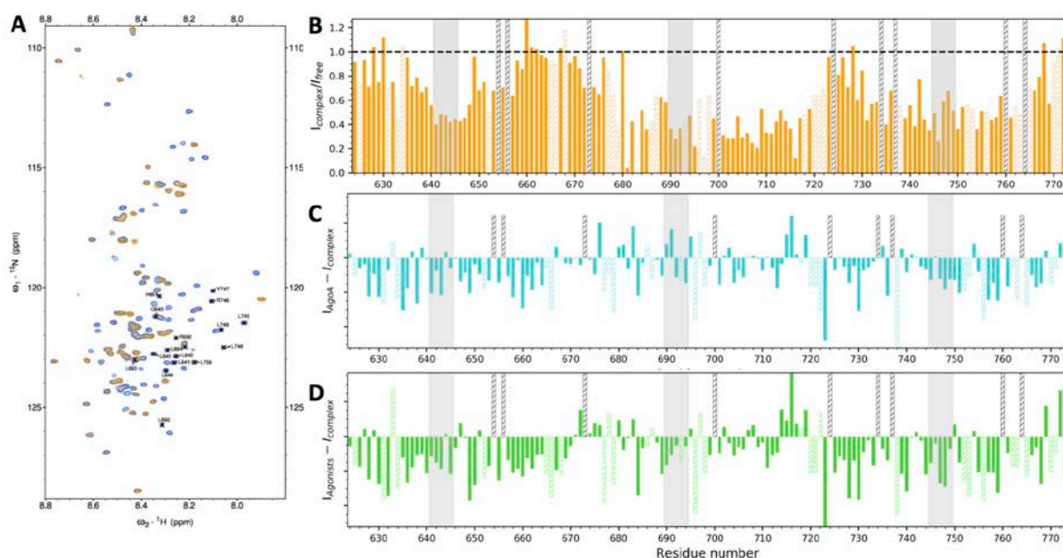
Figure 4. Interaction of TIF2 NRID with RXR/RAR LBDs and agonists effects. A) Superposition of 15 N-HSQC spectra of 5 \mu\text{M} of 15 N labelled TIF2 NRID in absence (blue) and in the presence (orange) of 6 \mu\text{M} of unlabelled RXR/RAR LBDs. Residues belonging to NR-boxes are indicated. B) Relative peak intensity ratios I_{\text{Complex}}/I_{\text{TIF2NRID}} between the two spectra presented in A. C) and D) Peak intensity differences between 15 N-HSQC spectra of RXR/RAR:TIF2 NRID complex (1.1:1) in the presence of 1.2 molar excess of RAR agonist AM580 (cyan, C); then followed by the addition of 1.2 molar excess of RXR agonist CD3254 (green, D). Bars highlighted in grey indicate NR-boxes. Dashed bars correspond to prolines (grey) or ambiguous and overlapped peaks (coloured).
