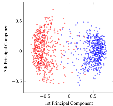
Figure 3: First and third (i.e. the ones with the highest MI with the sex class variable) principal components of original x -vectors from a subset of V2D ( 2 \times 5000 samples). The PCA have been trained on this subset. Females are in blue and males are in red.
