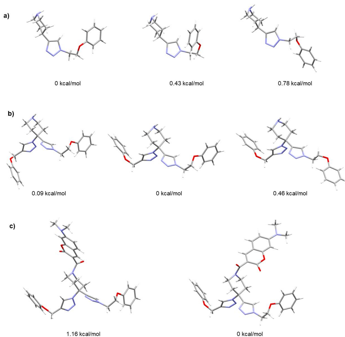
Figure 2. Most stable conformers of the three fragments with their relative energies: (a) phenyl-triazole, (b) di(phenyl-triazole) and (c) di(phenyl-triazole)-coumarin.
