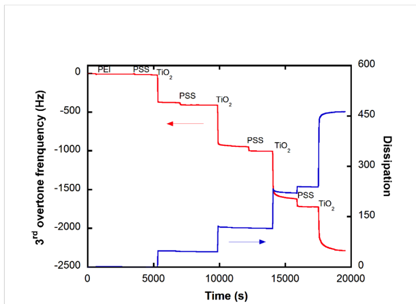
Figure 4 : Monitoring PEI/(PSS/TiO 2 ) n film construction by QCM-D at the 3 rd overtone. 4 PSS/TiO 2 layer pairs were deposited.
