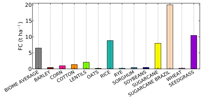
Figure 6. Fuel consumption (FC) for different US crop types as reported by McCarty et al. (2011), and Brazilian sugarcane (Lara et al., 2005). The grey bar corresponds to the biome-averaged FC value for crop residue burning as presented in this study.
