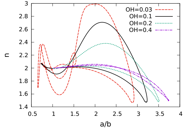
FIG. 4: Deformation pathway of a critically charged droplet as a function of the Ohnesorge number Oh . At the pointed tip appearance ( n = 1.5 ), the fissility is reduced from X = 1 to X = 0.64 .
