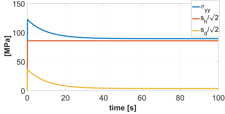
Figure 7: Transverse stress relaxation for a biaxial constant imposed strain state ( \varepsilon_{yy} = 0.01 , \varepsilon_{zz} = 0 )
