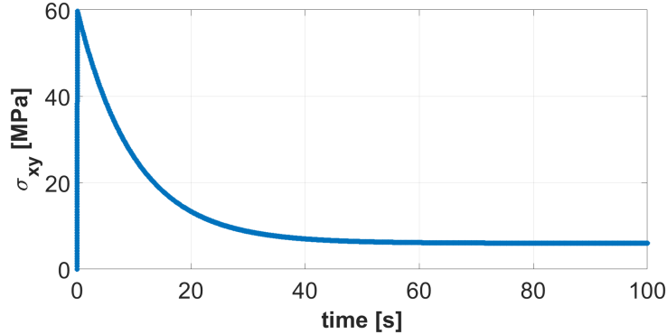
Figure 5: Shear stress relaxation for a constant imposed shear strain ( \varepsilon_{xy} = 0.005 )
