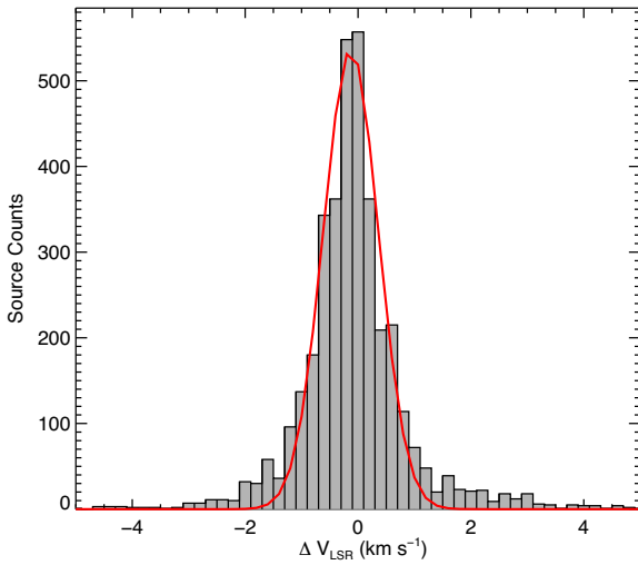
Figure 5. Histogram of the differences between previously assigned velocities (Urquhart et al. 2018) and the velocities obtained from analysis of the SEDIGISM data discussed in this paper. The red curve shows the Gaussian fit to the distribution, which has a FWHM of 1.1 km s -1 . The bin size is 0.2 km s -1 .
