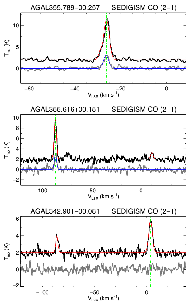
Figure 3. Examples of the ^{13}\text{CO} (black line) and \text{C}^{18}\text{O} (grey) spectra extracted towards three dense clumps identified from the ATLASGAL survey; the former is offset by 2 K from zero intensity. The results of the automatic Gaussian fitting are overlaid in red and blue and the velocity assigned to the clump is indicated by the green vertical dash-dotted line.
