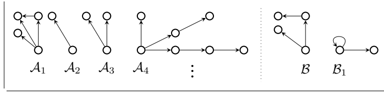
Fig. 3. The sets of frames \mathbf{A} = \{\mathcal{A}_1, \mathcal{A}_2, \mathcal{A}_3, \mathcal{A}_4\} and \mathbf{B} = \{\mathcal{B}, \mathcal{B}_1\} .
