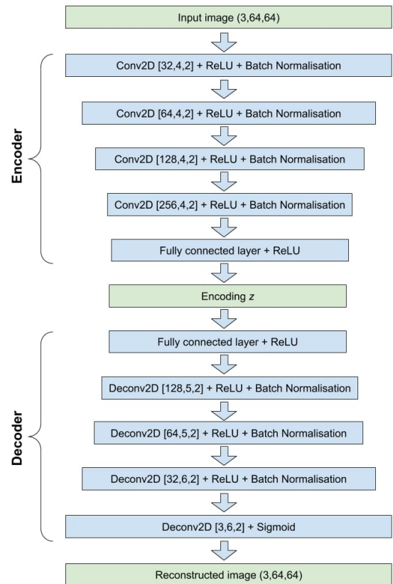
Fig. 9. Backbone architecture of the Auto-Encoder used in this work. Conv2D stands for the 2D convolution operation with [number of kernels, size of kernels, stride] parameters, ReLU for Rectified Linear Unit activation function, Deconv2D for the 2D deconvolution operation with [number of kernels, size of kernels, stride] parameters, and Sigmoid for the sigmoid activation function. (1-column image).
