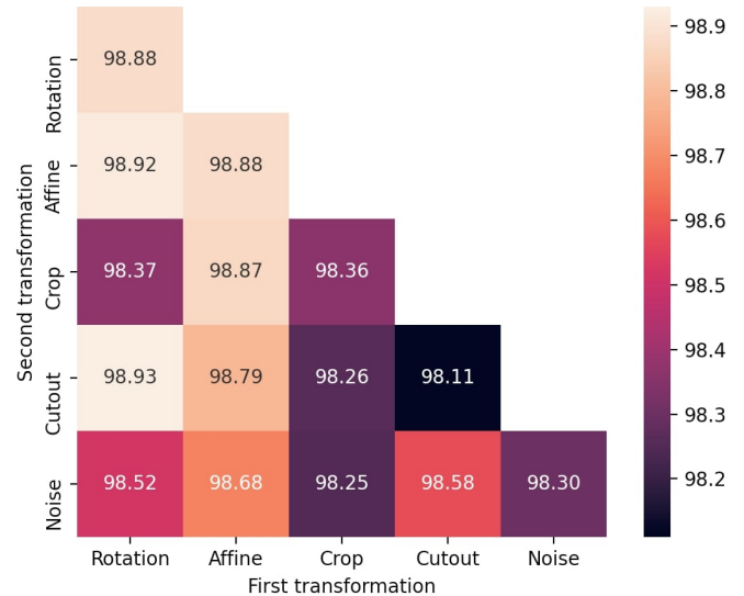
Fig. 11. Accuracies obtained for different data augmentations on the MNIST dataset. (1-column image).
