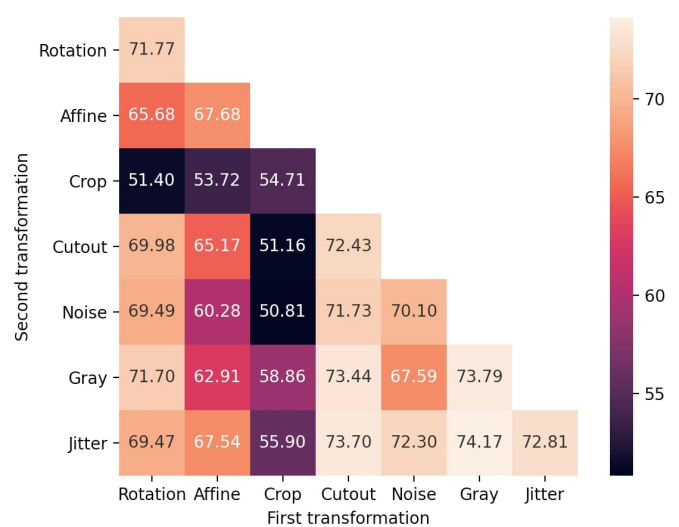
Fig. 13. Accuracies obtained for different data augmentations on the SVHN dataset. (1-column image).
