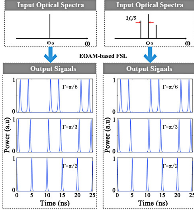
Fig. 4. EO-AM FSL under the integer Talbot condition. Simulation output power with (left) single frequency and (right) multi-tone input. Double-pulse operation depends on the EO bias ( \Gamma ) but there is no frequency-to time mapping.
