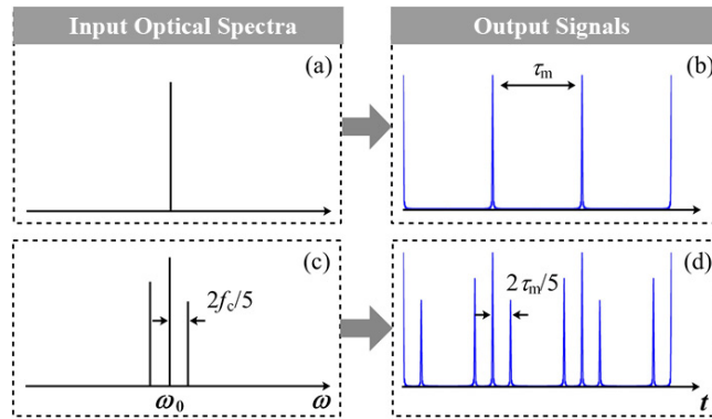
Fig.2 FTM process in the AO-FSL. (a) Single-frequency input yields the pulsed output in (b). (c) Multi-tone input yields the output signal in (d) that maps the input spectrum.
