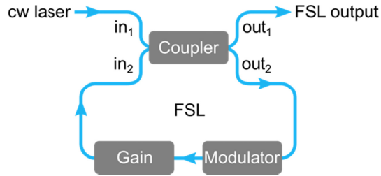
Fig.1 Sketch of the FSL. The modulator induces pure frequency-translation (AO), or dual-sideband generation in either amplitude (EO-AM), or phase (EO-PM) cases.
